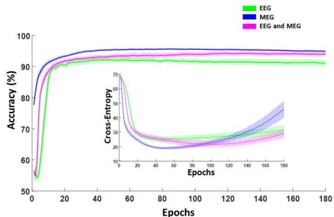
Fig. 3. Average (and related standard error), 10-fold cross-validated, accuracy (evaluated after an ArgMax operation on the SoftMax output) and cross-entropy of the CNN in classifying brain or artefact ICs as a function of training epoch. The CNN was trained on three datasets: standalone EEG (green), standalone MEG (blue), combined EEG and MEG (magenta).
