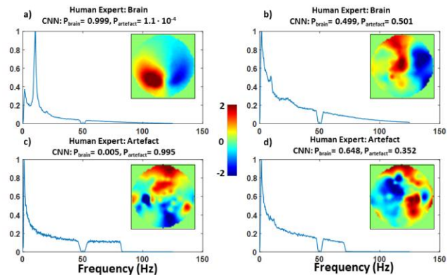
Fig. 6. Examples of CNN input ICMAPs and ICSPECTs classified by human experts as either brain activity (a and b), or artefact (c and d). The CNN correctly classified the ICs reported on the left side of the figure (a and c), and erroneously classified the ICs reported on the right side of the figure (b and d).
