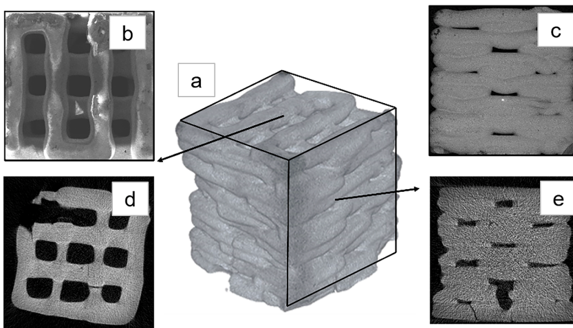
Fig. 2. Morphometric characterization of the BCP scaffold. a Three-dimensional (3D) model of the BCP scaffold through X-ray micro-computed tomography (X \mu CT), with b-d top faces and c-e lateral faces showing different patterns; b-c SEM micrographs; d-e single slices of X \mu CT reconstructions; (right panel) X \mu CT data.
