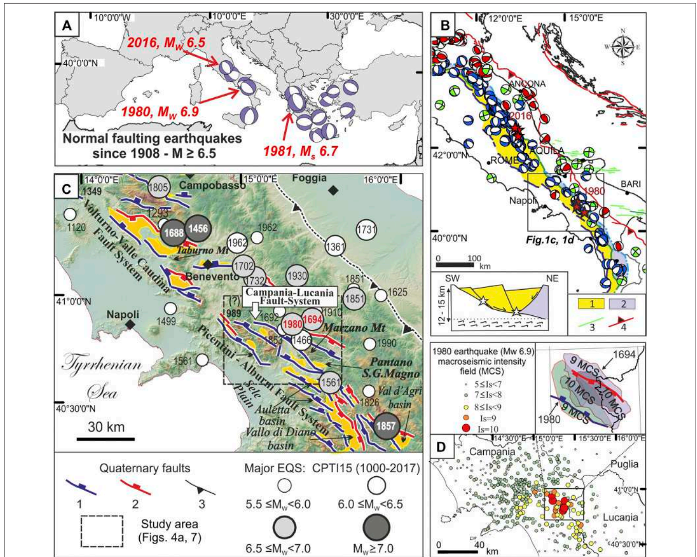
FIGURE 1 | The Campania-Lucania 1980 earthquake in the Mediterranean seismotectonic context. (A) Mediterranean normal faulting earthquakes with M \geq 6.5 since 1908 derived from the World Stress Map database (Heidbach et al., 2018). (B) The Italian earthquake focal mechanisms ( M_w \geq 4.0 ) from 1980 to 2015 (Montone and Mariucci, 2016); red stars represent the mainshocks of 2016/2017 Central Italy and 1980 Campania-Lucania seismic sequences. The background colors indicate the extensional seismotectonic provinces as in Lavecchia et al., 2021: Key: 1 = Extensional seismogenic province; 2 = Deep extensional seismogenic province; 3 = right-lateral strike-slip faults within the Adriatic foreland; 4 = Active outer thrust system; The sketch in the lower left corner represents the simplified model of the Apennine extensional system as in Lavecchia et al., 2011. (C) Active faults in Southern Italy (after Adinolfi et al., 2015) with major historical and instrumental earthquakes from Parametric Catalogue of Italian Earthquakes, CPTI15 v2.0 (Rovida et al., 2019). Key: 1, east-dipping normal faults; 2, west-dipping normal faults; 3 thrust faults. (D) 1980 earthquake macroseismic field from the Italian Macroseismic database DBMI15 v2.0 (Locati et al., 2019). The inset in the right upper corner represents the contour of IX and X MCS intensity of the 1694 and 1980 earthquakes.
