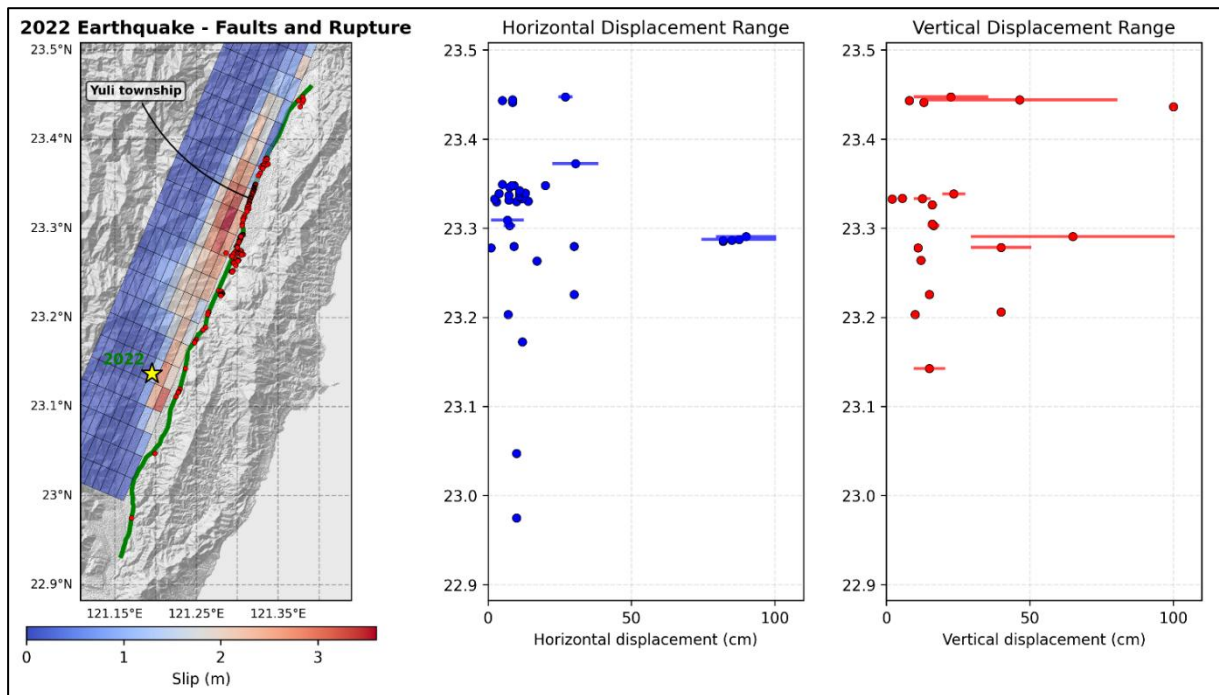
Figure 2-17: Comparison of the 2022 Chihshang earthquake surface ruptures with a proposed finite fault model (USGS, 2022).
