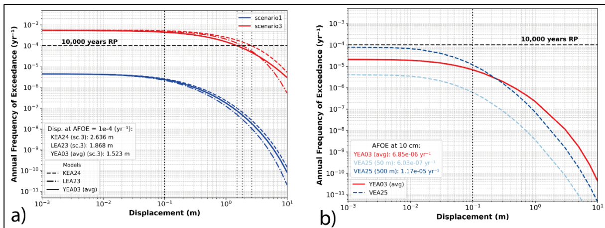
Figure 3-33: Fault displacement hazard models variability a) for principal faulting on the East Crati fault (Rovito town); b) for distributed faulting in Castrovillari.
