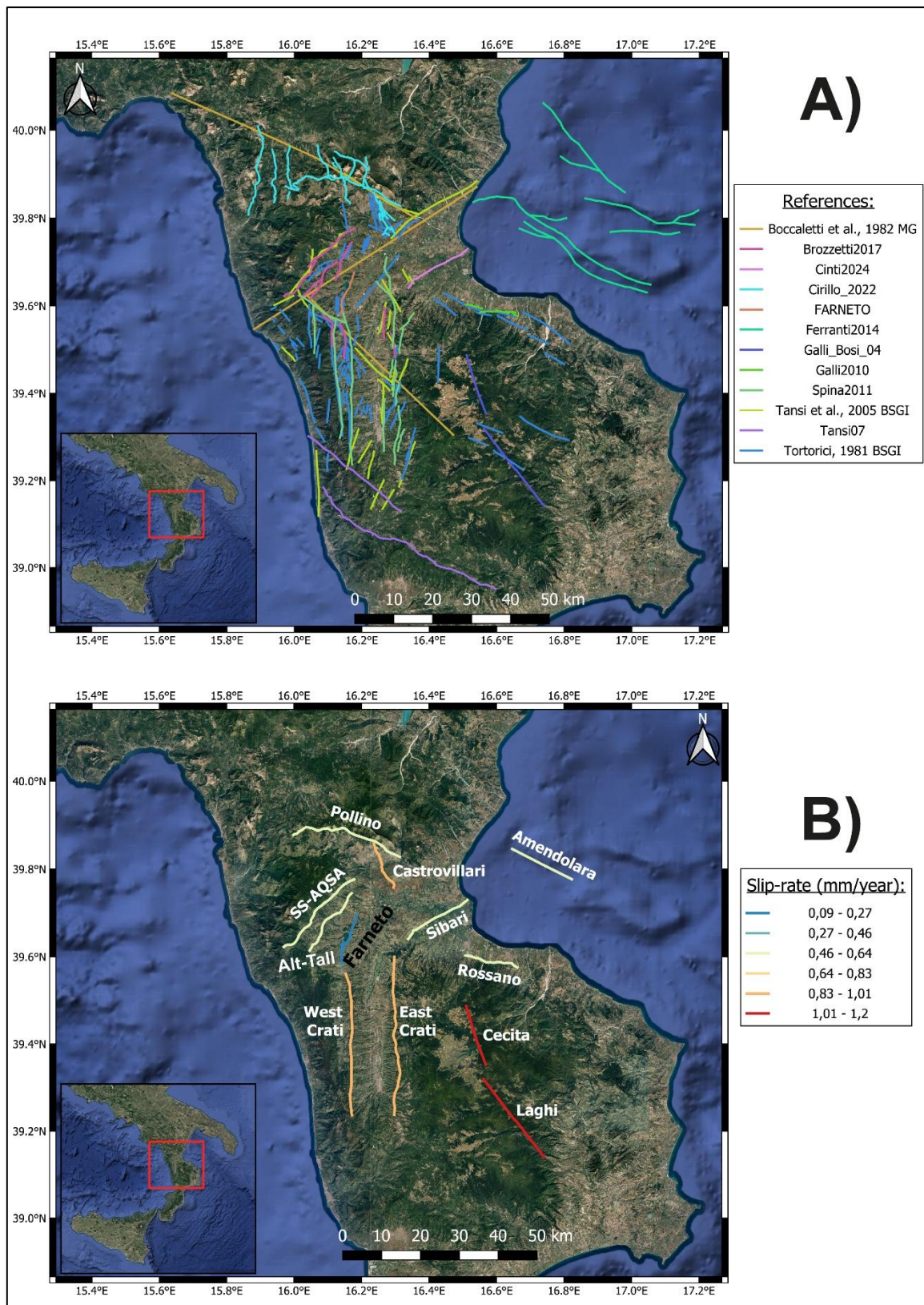
Figure 3-18: Refined active and capable faults in Northern Calabria. A) Traces of active faults collected in the literature; B) Surface expression of the final simplified seismotectonic model (SS-AQSA: San Sosti – Acquaformosa system; Alt-Tall: Altomonte-Tallarito system).
