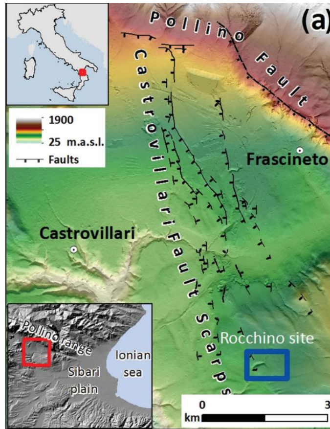
Figure 3-9: Castrovillari fault system (from Cinti et al., 2015; Figure 1a)
