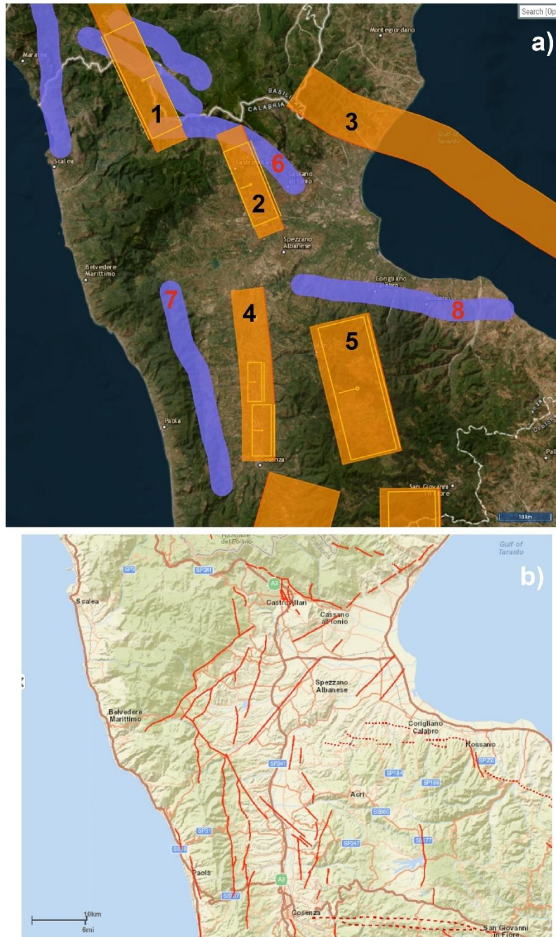
Figure 3-7: Seismogenic sources and capable faults in northern Calabria. a) Seismogenic sources from the DISS database (Basili et al., 2008; DISS Working Group, 2025), with: 1- Rimendiello-Mormanno (ITCS038); 2- Pollino (ITCS033); 3- Amendolara (ITCS041); 4- Crati Valley (ITCS015); 5- Cecita lake (ITCS176). In purple, the debated sources, with: 6- Pollino (ITDS009); 7- Catena Costiera (ITDS030); 8- Rossano (ITDS028). b) Capable faults from ITHACA (ITHACA Working Group, 2019).
