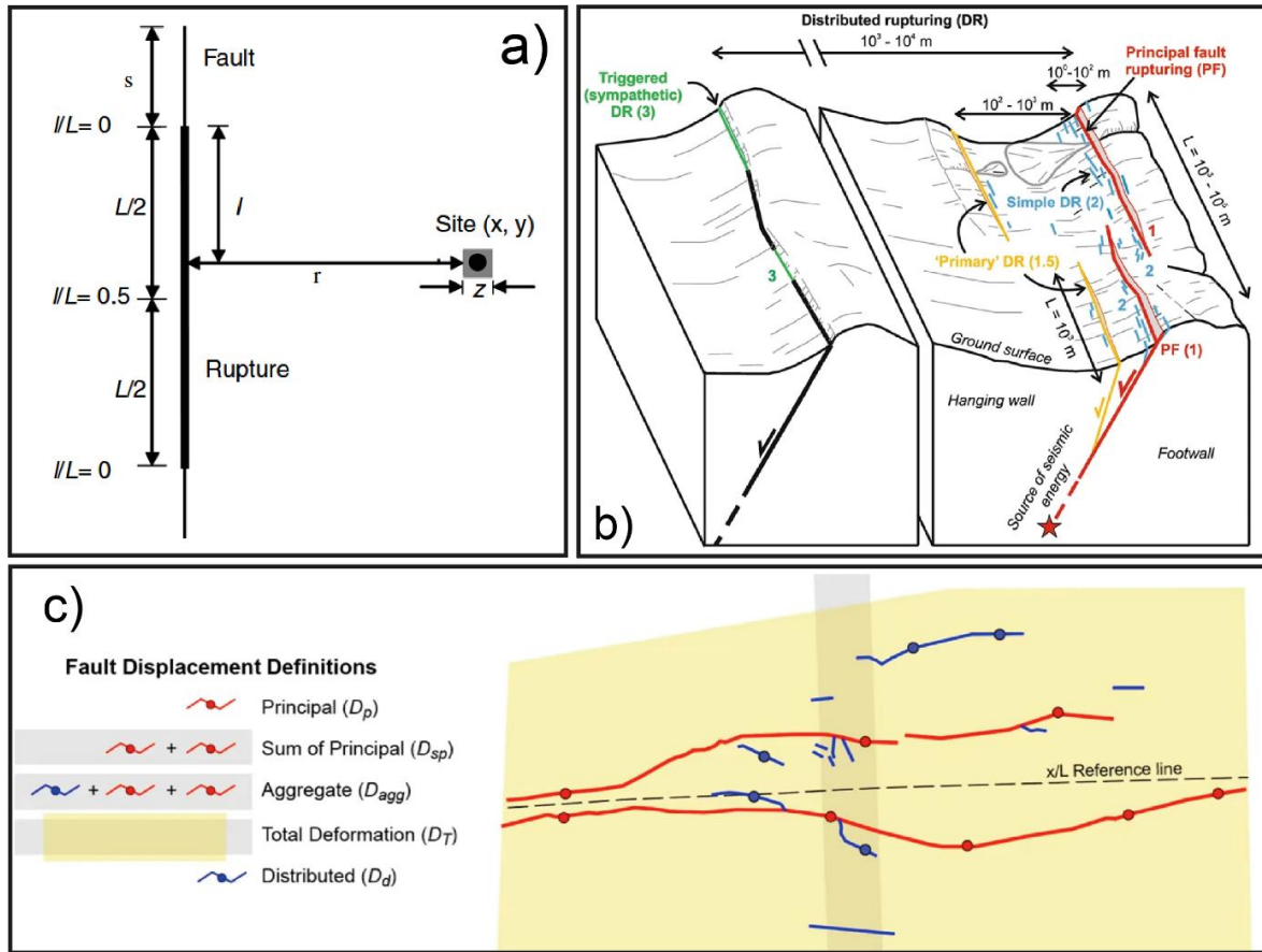
Figure 1-12: Fault displacement metrics and definitions proposed in literature. a) Distance variables definition (taken from Petersen et al., 2011; Figure 1); b) New terminology with variable fault ranking in a normal faulting case (taken from Nurminen et al., 2022; Figure 1a); c) Definitions used for more complex fault geometries at the surface (taken from Thompson, 2024): “Sum of principal” accounts for sub-parallel principal faulting: “Aggregate” displacement is the sum of the principal and the distributed faulting, as used by Youngs, within an orthogonal area relative to the main fault.
