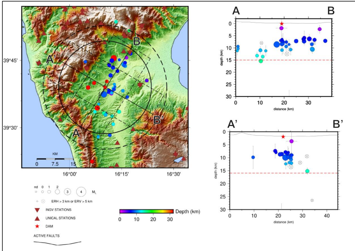
Figure 3-5: Relocated dataset using Hypo71 software.
