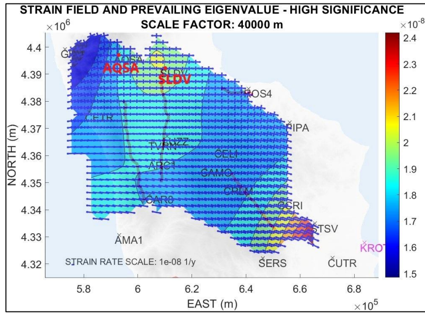
Figure 3-23: Maximum strain field obtained from GNSS data in northern Calabria. The Acquaformosa (AQSA) and San Lorenzo del Vallo (SLDV) stations are represented on the map. The strain field between those two stations is around 1.9 \text{ E-}8 \text{ yr}^{-1} .
