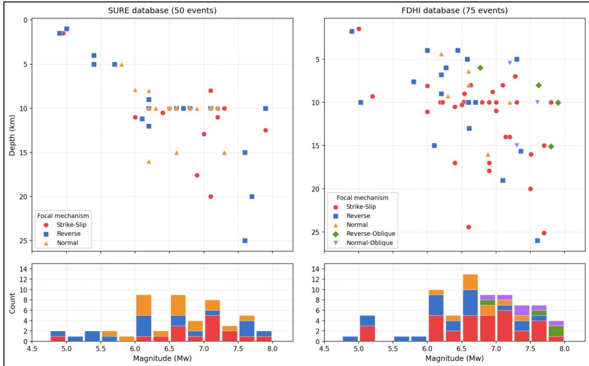
Figure 1-11: Earthquake magnitude and epicentral depth distributions using data from the SURE 2.0 and FDHI databases. Events with no reported epicentral depth are excluded.
