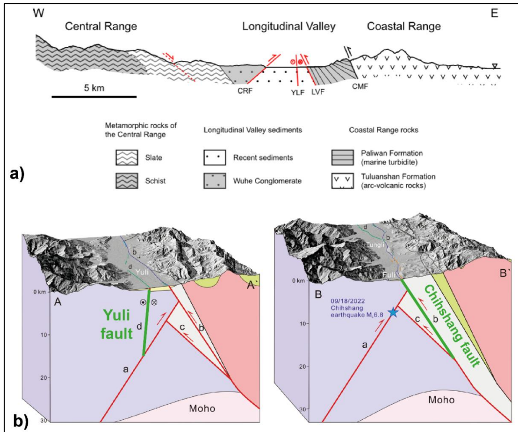
Figure 2-2: Geometry of the southern part of Longitudinal Valley fault system: a) Schematic geologic cross-section of the LVF (from Shyu et al., 2006; Figure 5). b) Cross-sections illustrating the tectonic setting at two different places along the LVF. The positions of the two cross-sections AA' and BB' are indicated in Figure 2-14 (modified from Chen et al., 2024).
