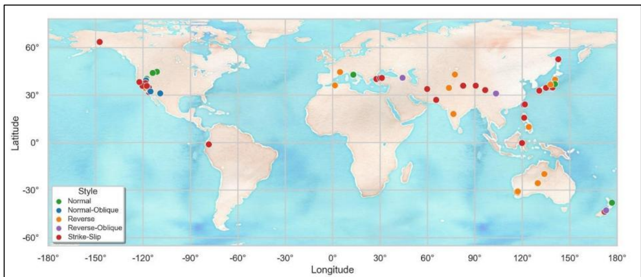
Figure 1-10: Location and style of faulting of the FDHI database earthquakes (from Sarmiento et al., 2021; Figure 1.1).
