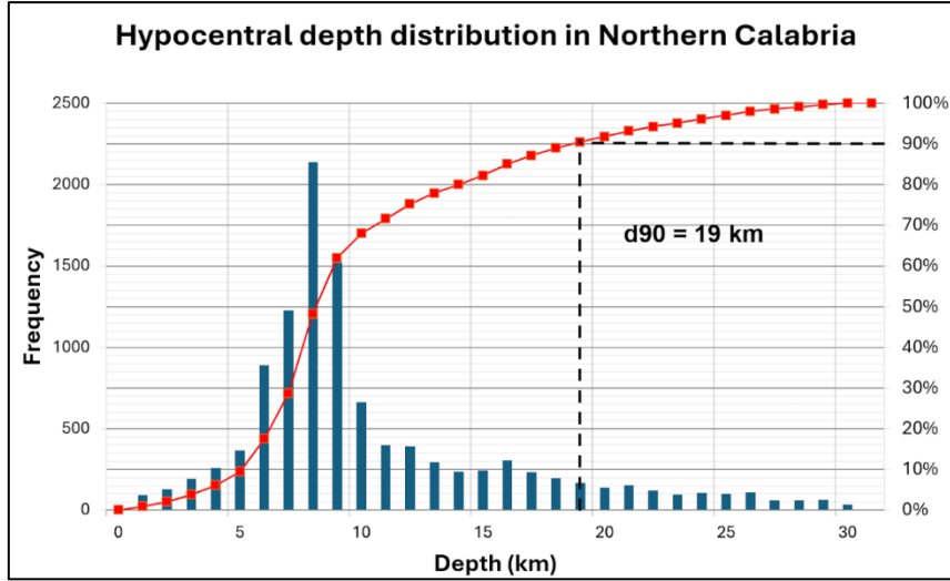
Figure 3-21: Hypocentral depth distribution in northern Calabria, using the CLASS catalogue (Latorre et al., 2022). The blue bars represent the frequency distribution of hypocentral depths, the red line is the cumulative distribution function, and the black dashed line represents the d90 depth threshold, below which 90% of earthquakes occur.
