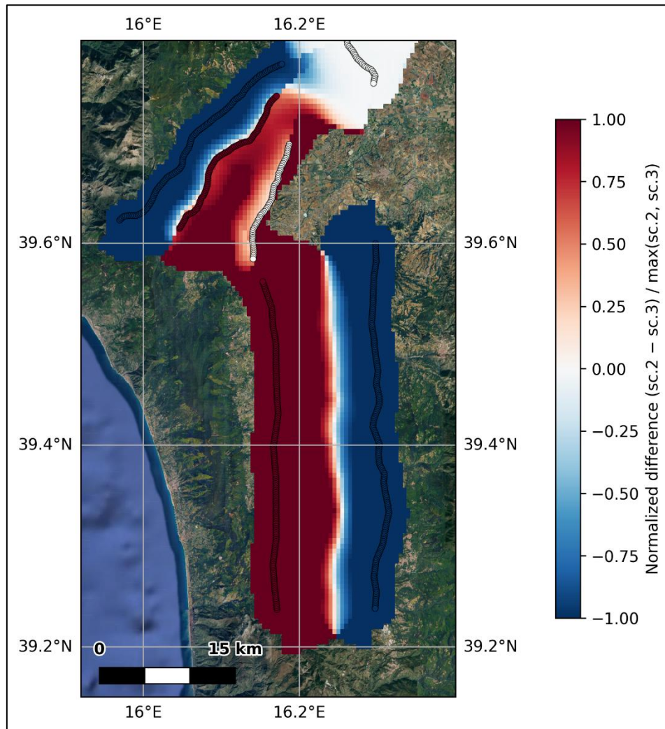
Figure 3-32: Differences map between scenario 2 and scenario 3. Circles represent the sampled sites along the fault traces.
