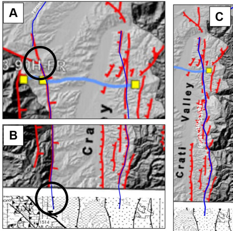
Figure 3-20: Details regarding the construction of the final fault sources in the Crati Valley: in blue, the proposed simplification with respect to the segments mapped on the surface. A: northern sector of the western system, taken from Spina et al., 2011; B: western Crati, southern part, from Spina et al., 2011 and Tansi et al., 2007 for the termination; C: eastern Crati source, from north to south.
