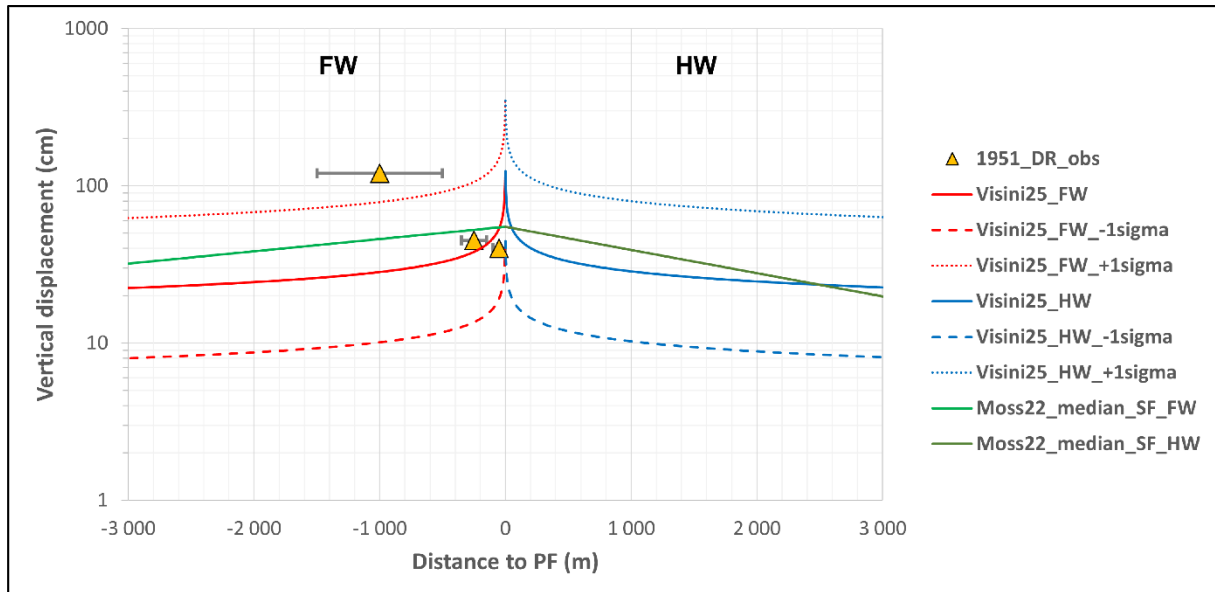
Figure 2-9: Comparison of the distributed vertical displacement observed during the 1951 Hualien earthquake with empirical regressions from MEA22 (Moss22) and VEA25 (Visini25) (HW: hanging wall, FW: foot wall).
