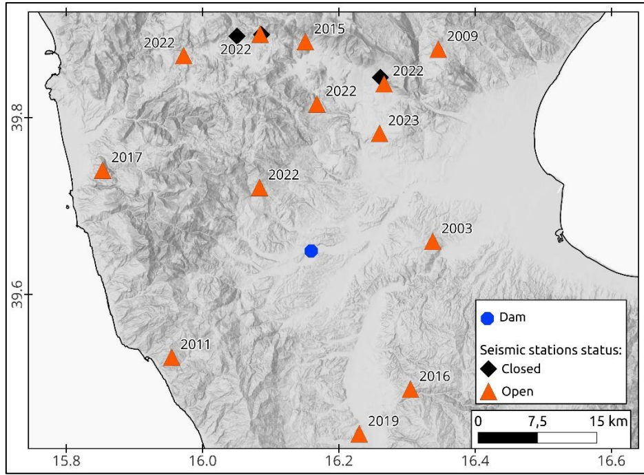
Figure 3-3: Seismic network around the Farneto dam in 2023, in northern Calabria.
