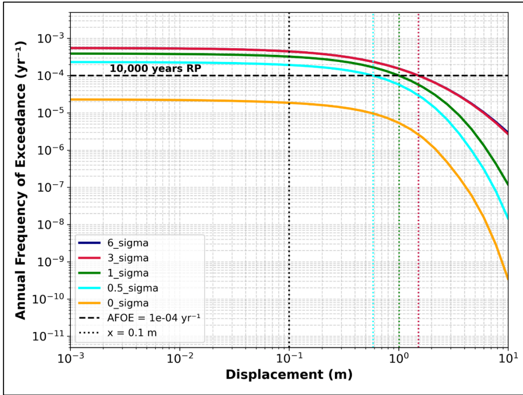
Figure 3-34: Sigma truncation exploration at the Rovito site (using YEA03 only). The 6 sigma curve (the standard value set for our calculations) coincides with the 3 sigma truncation curve.
