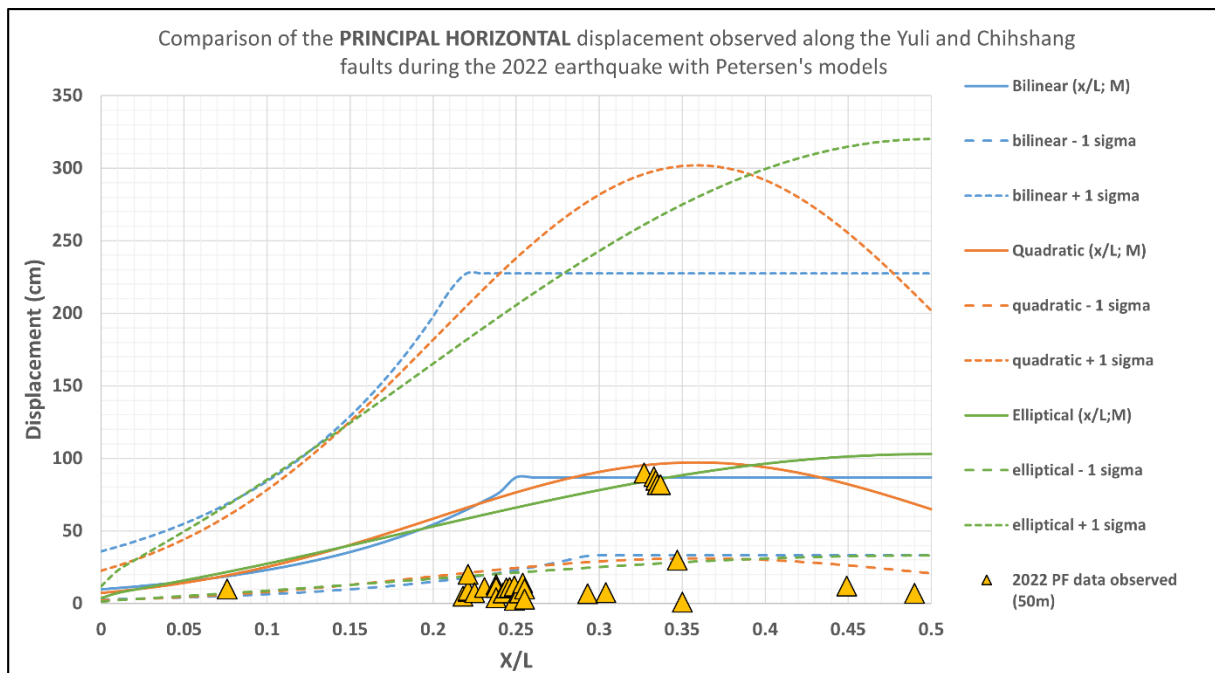
Figure 2-20: Comparison of the principal horizontal displacement observed along the Yuli and Chihshang faults during the 2022 earthquake with the PEA11 models.
