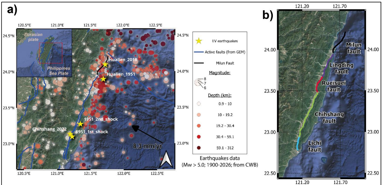
Figure 2-1: Map of the Longitudinal Valley fault (LVF) system. a) Seismic activity in the Longitudinal Valley in Taiwan during the last century. The active faults are from Styron and Pagani (2020) and Shyu et al. (2020). b) Details of the fault segments forming the LVF.
