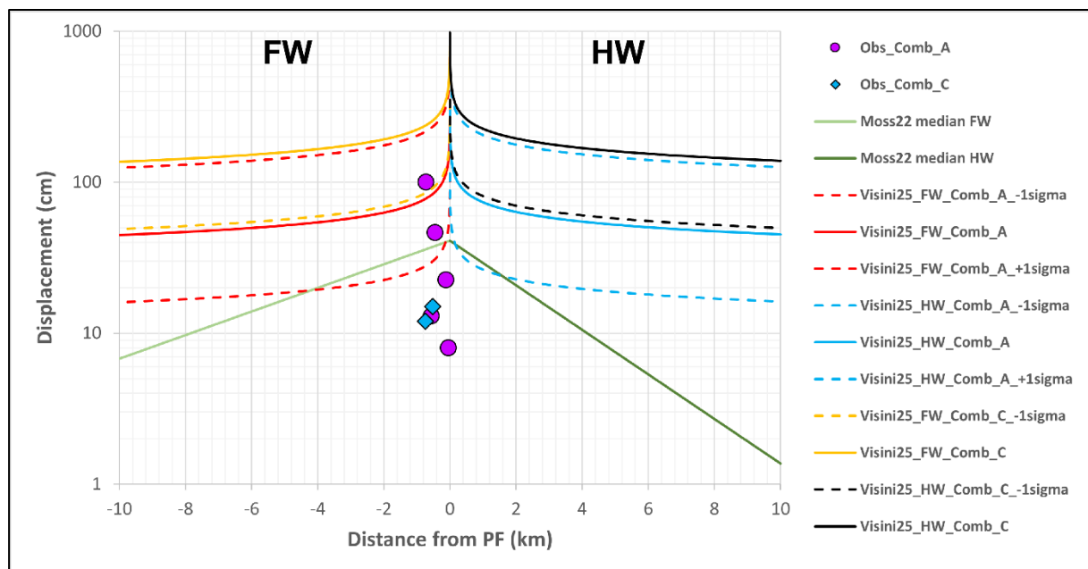
Figure 2-23: Comparison of the distributed vertical displacement observed during the 2022 Chihshang earthquake with empirical regressions from MEA22 (Moss22) and VEA25 (Visini25) (HW: hanging wall, FW: foot wall).
