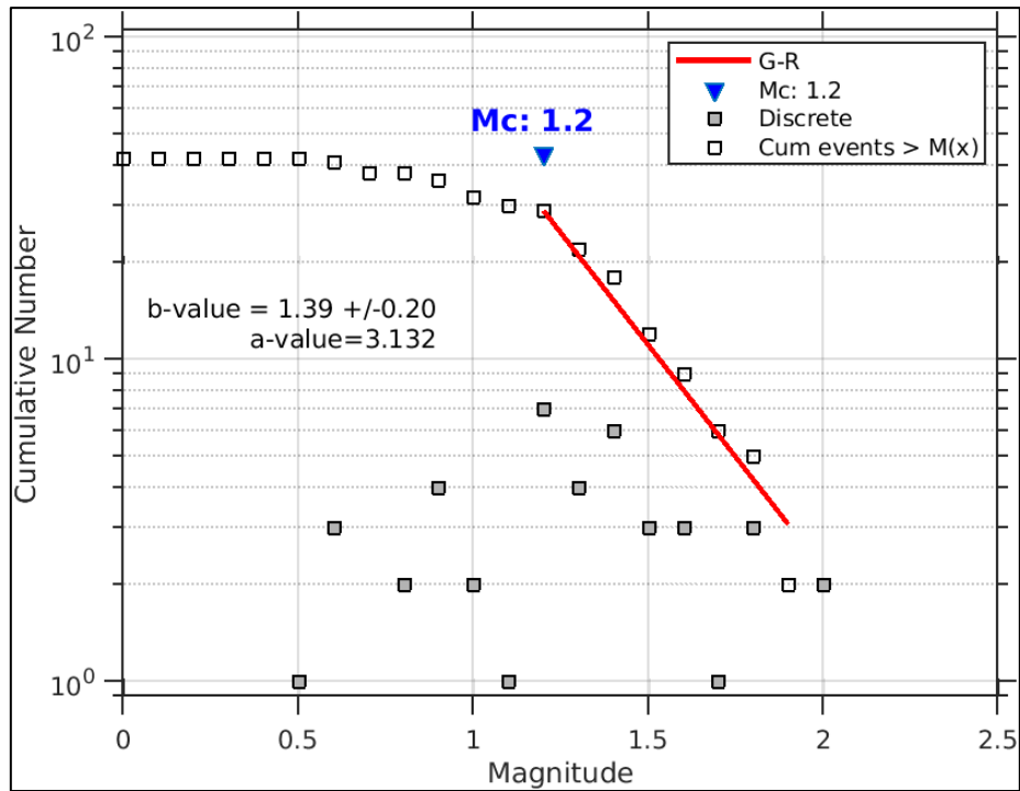
Figure 3-6: Gutenberg-Richter law computed from the 42 events of the relocated events dataset.
