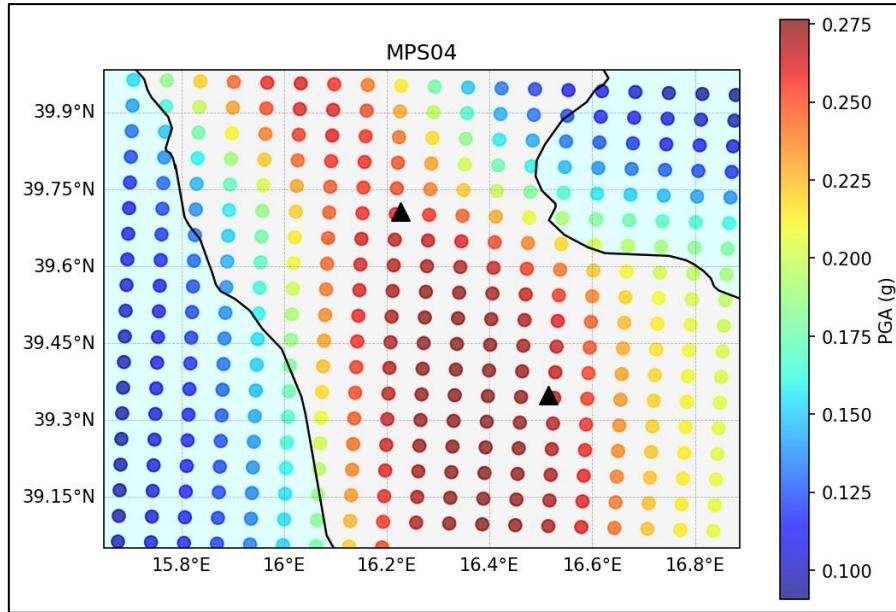
Figure 3-26: Northern Calabria hazard map representing the PGA having 10% chance to be exceeded in the next 50 years. The triangles represent the two sites chosen for hazard curves comparison. Data from MPS04 (Meletti et al., 2006).
