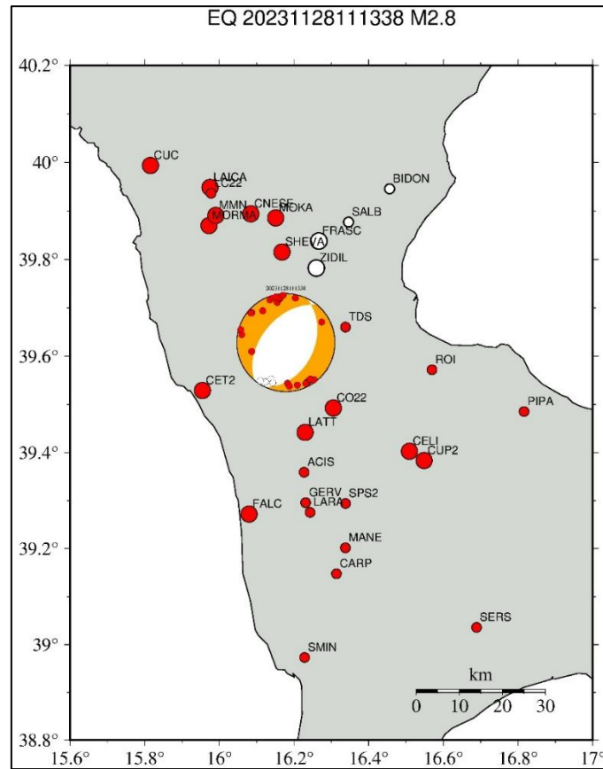
Figure 3-19: Focal mechanism of the Mw 2.8 November 2023 earthquake in the central Crati Valley area. In red, are shown the stations used to compute the focal mechanism.
