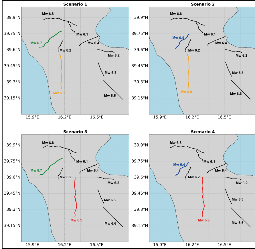
Figure 3-24: Geometric sketch of the four scenarios used in our study (alternative fault pairs are shown in red and yellow for the East Crati and West Crati faults, and in green and blue for the San Sosti and Altomonte-Tallarito faults, respectively).
