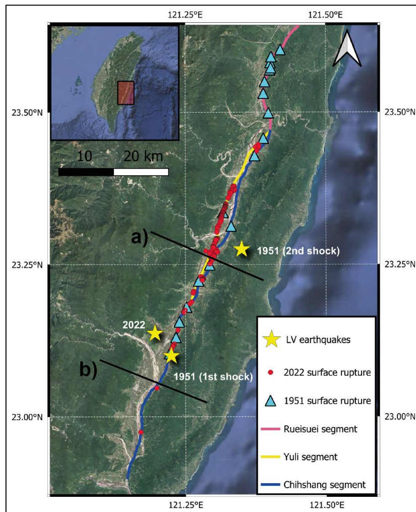
Figure 2-14: Location of the surface rupture data collected for the 1951 and 2022 earthquakes in the southern part of the LVF. The solid black lines represent the cross-sections of Figure 2-2.
