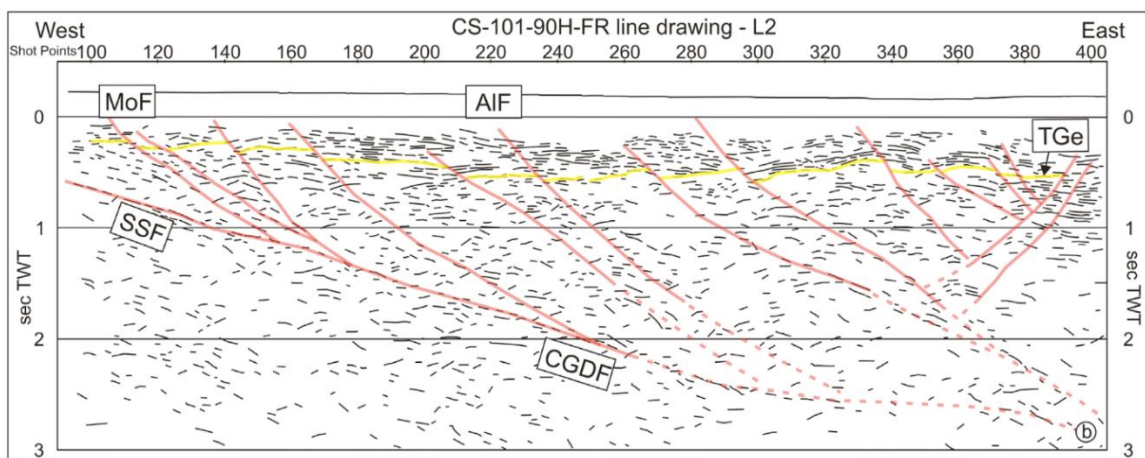
Figure 3-13: Interpretation of a seismic line in the northern part of the Crati valley (Line L2 in Figure 3-12; from Brozzetti et al., 2017a)
