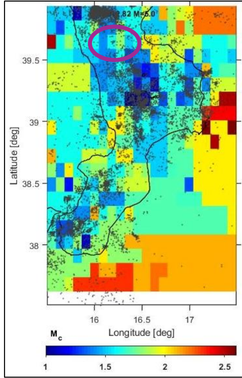
Figure 3-2: Magnitude of completeness of the ISIDe catalogue. The area of interest is represented by the purple ellipse.
