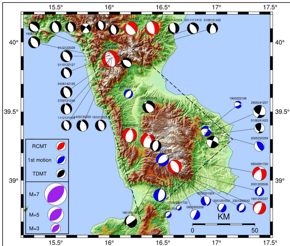
Figure 3-22: Map of the focal mechanisms collected in northern Calabria (red: RCMT database; black: TDMT database; blue: 1st motion polarity data from Chiappetta and La Rocca, (2023) and Ciaccio et al. (2021)).
