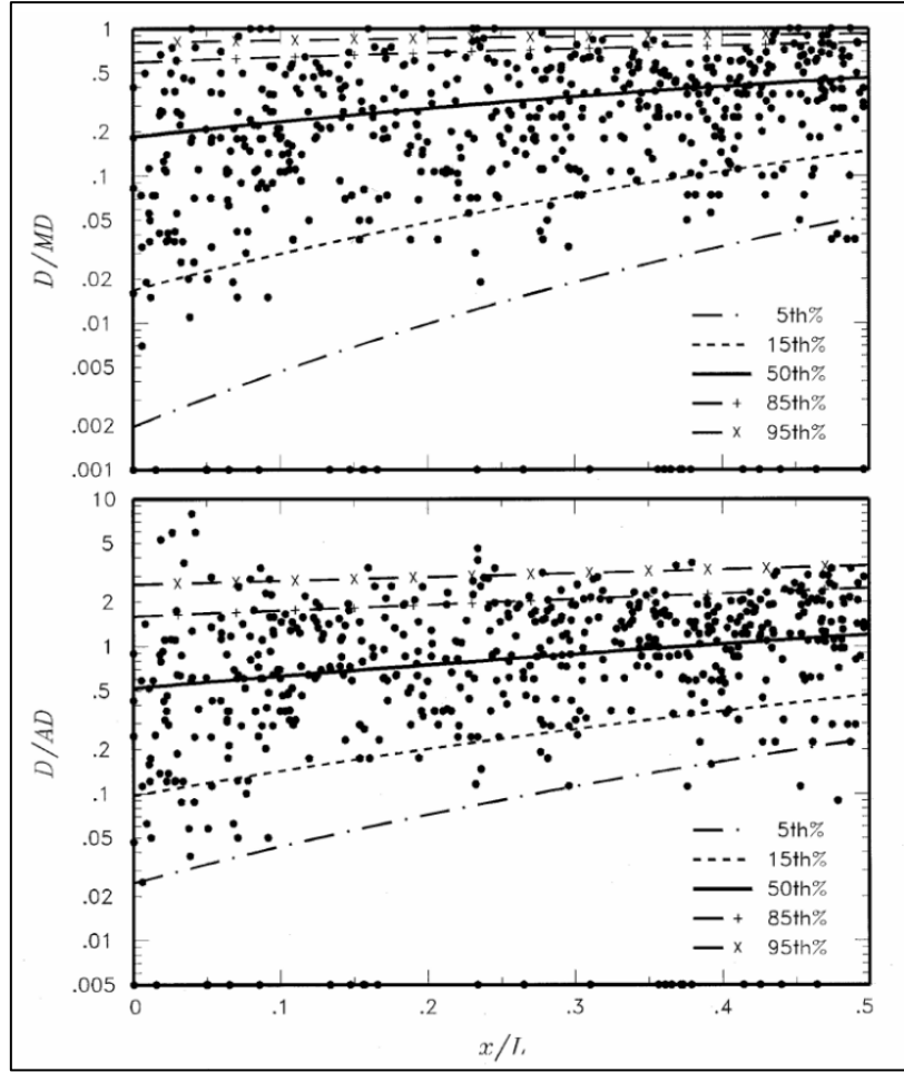
Figure 1-4: Normalised displacement distributions along the principal fault using data from McCalpin and Slemmons (1998). Top: D/MD using a beta distribution. Bottom: D/AD distribution using a gamma distribution (taken from Youngs et al., 2003; Figure 7)
