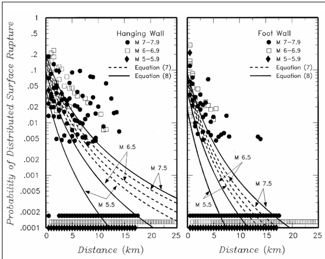
Figure 1-6: Conditional probability of occurrence of distributed rupture (taken from Youngs et al., 2003, Figure 9).
