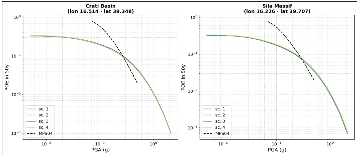
Figure 3-28: Probability of exceedance in 50 years comparison for two sites in northern Calabria (Crati Basin on the left and Sila Massif on the right side).
