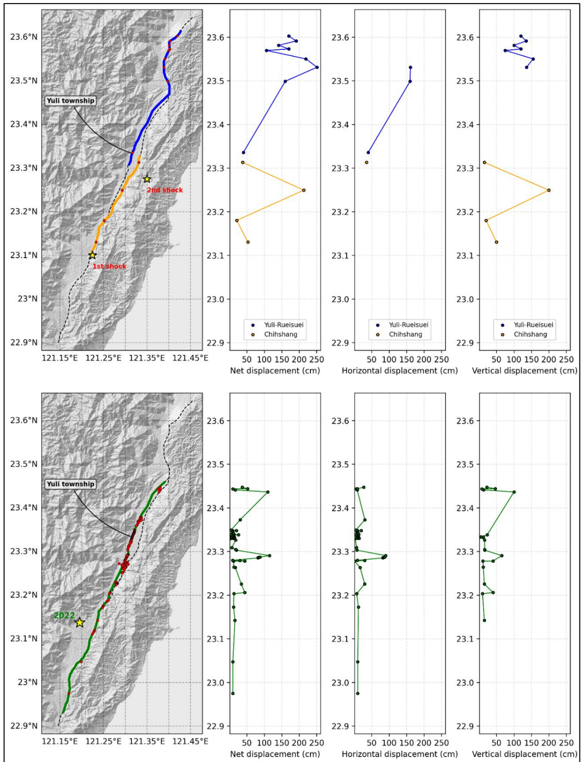
Figure 2-15: Spatial slip component comparison of the surface ruptures observed during the 1951 and 2022 earthquakes. The upper panels show the 1951 events displacement component comparisons. The lower panels represent the same comparisons for the 2022 earthquake. On the left maps, in blue: Yuli-Rueisuei combined rupture in 1951; in yellow: Chihshang rupture in 1951; in green: Yuli-Chihshang combined rupture in 2022.
