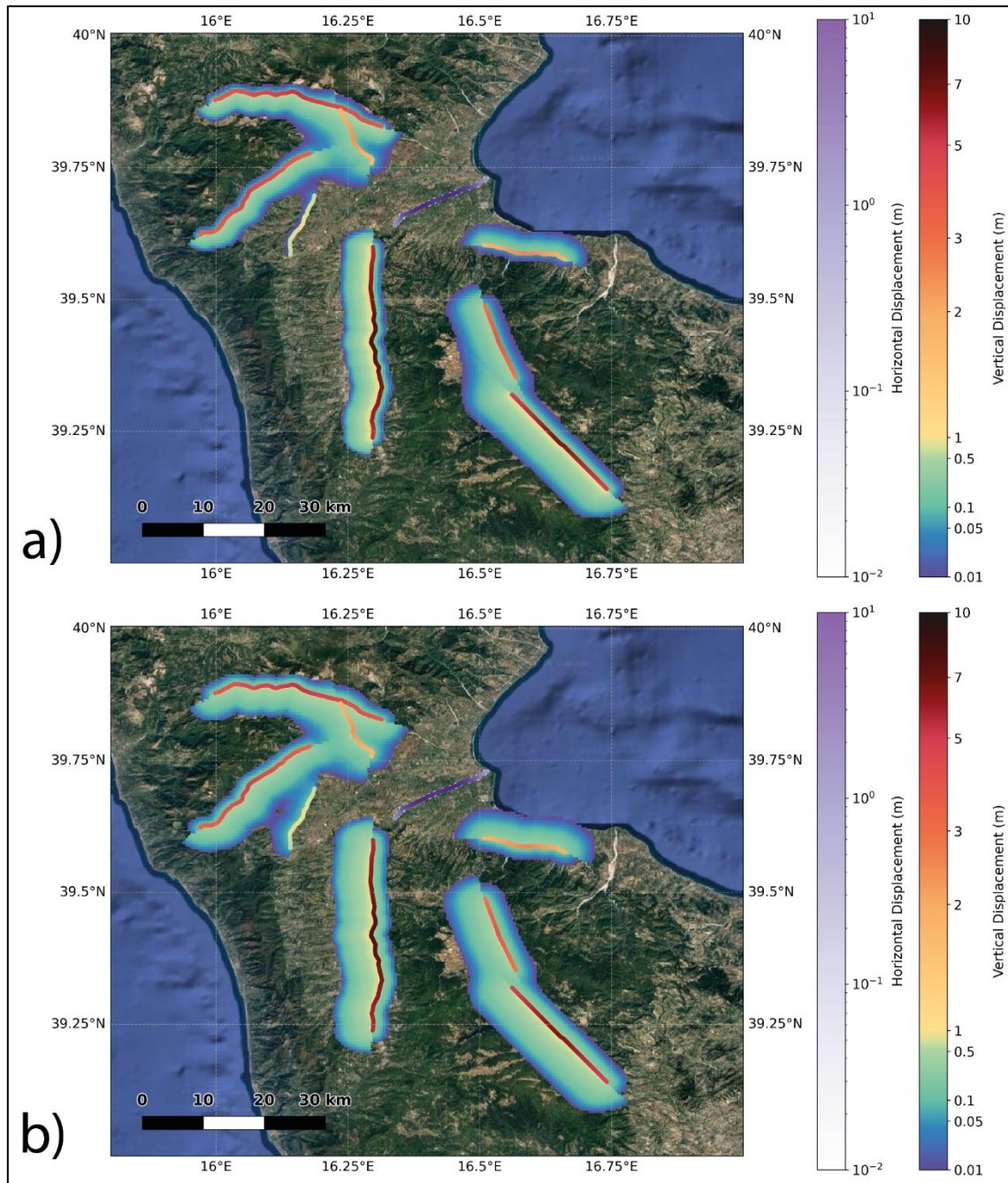
Figure 3-30: Fault Displacement Hazard maps comparison between YEA03 (frame a) ) and VEA25 (frame b) ) for scenario 3 and a return period of 100 ka. The colour scale bars are different for horizontal and vertical displacements, representing respectively strike-slip and normal faults.
