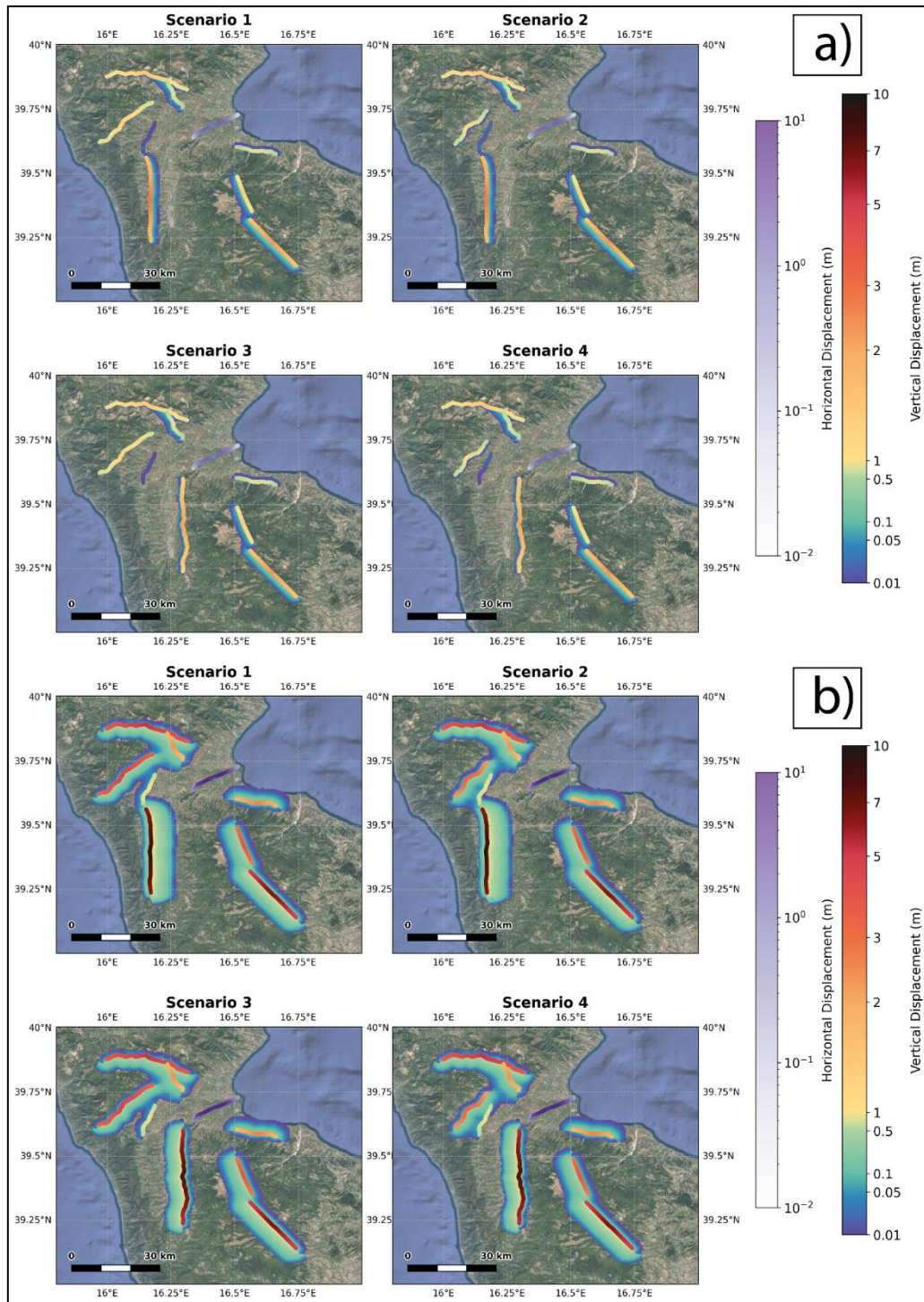
Figure 3-31: 4 scenario fault displacement hazard maps using YEA03 and VEA25 models equally weighted, a) for a return period of 10 ka, and b) for 100 ka. Colour scale bars as in the previous figure.
