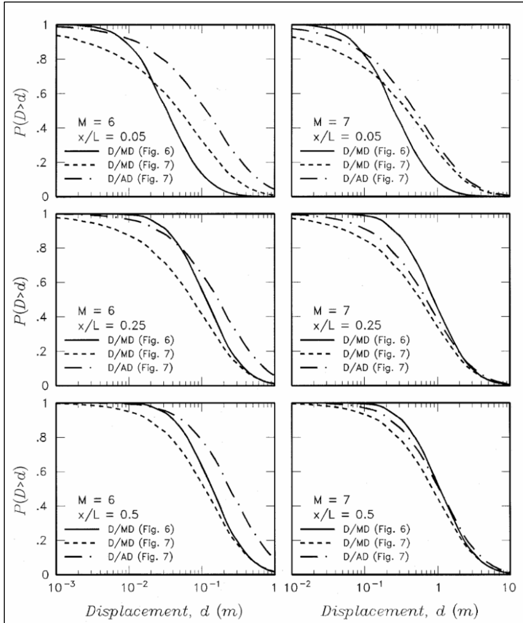
Figure 1-5: Conditional probability of exceedance for principal faulting, for various earthquake magnitude and x/L values (taken from Youngs et al., 2003; Figure 8).
