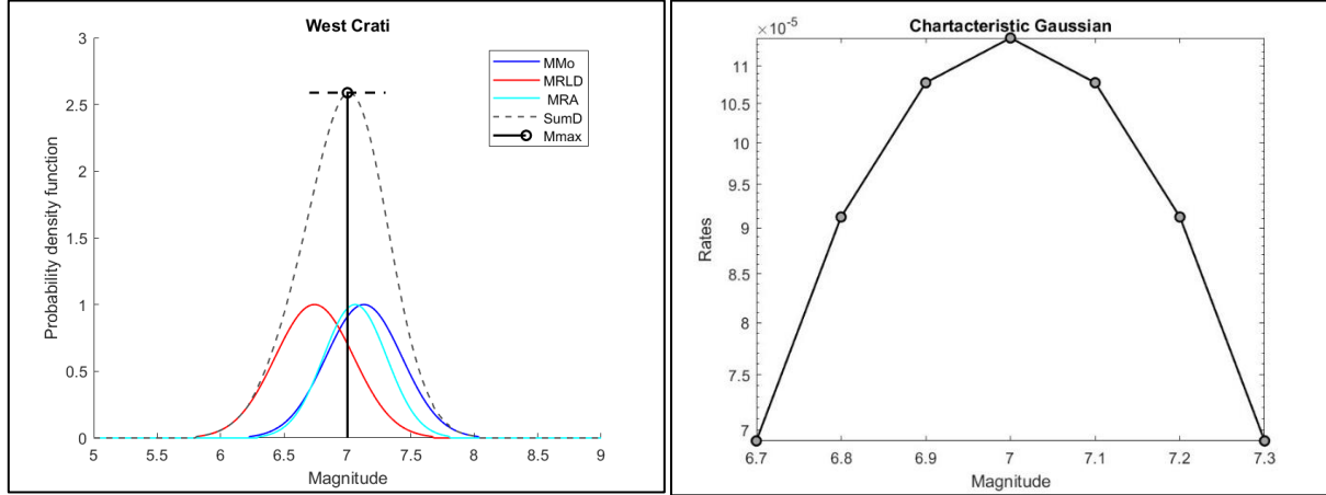
Figure 3-25: MFD characterisation for the West Crati source. On the left: Magnitude estimations using various scaling relationships from Wells and Coppersmith, (1994). MMo: Moment magnitude; MRLD: Magnitude from rupture length at depth; MRA: Magnitude from rupture area; SumD: sum of the magnitude distributions; Mmax: Averaged maximum magnitude expected. On the right: activity rate distribution.
