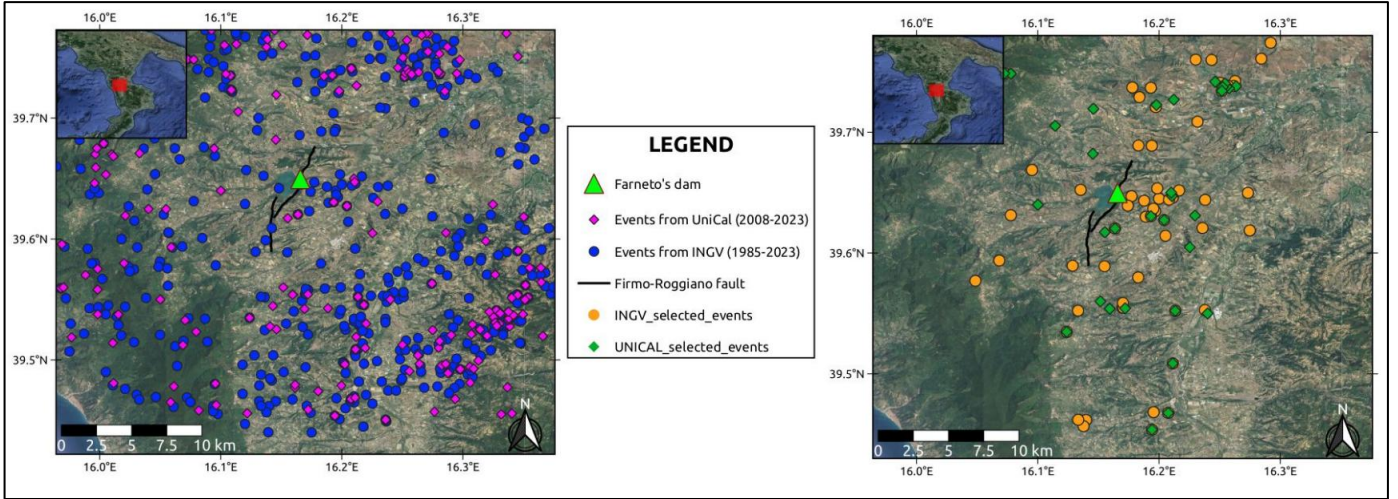
Figure 3-4: Earthquake data collection around the Farneto dam. a) All events in the 20 km study area. b) All events for which waveforms could be found.
