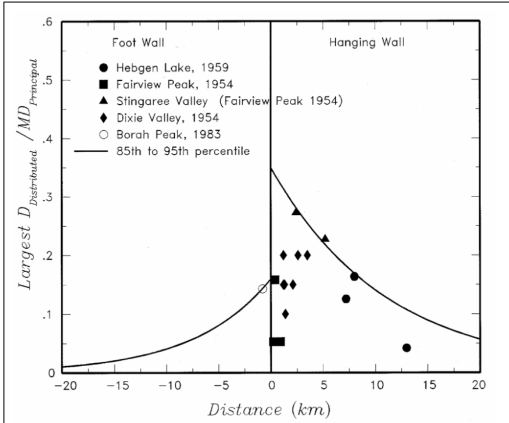
Figure 1-7: Distributions of the D_{distributed}/MD ratio with distance from the main fault, for the foot wall (left) and the hanging wall (right). Data from De Polo (1994) used to calculate them are also plotted. (taken from Youngs et al., 2003, Figure 11).
