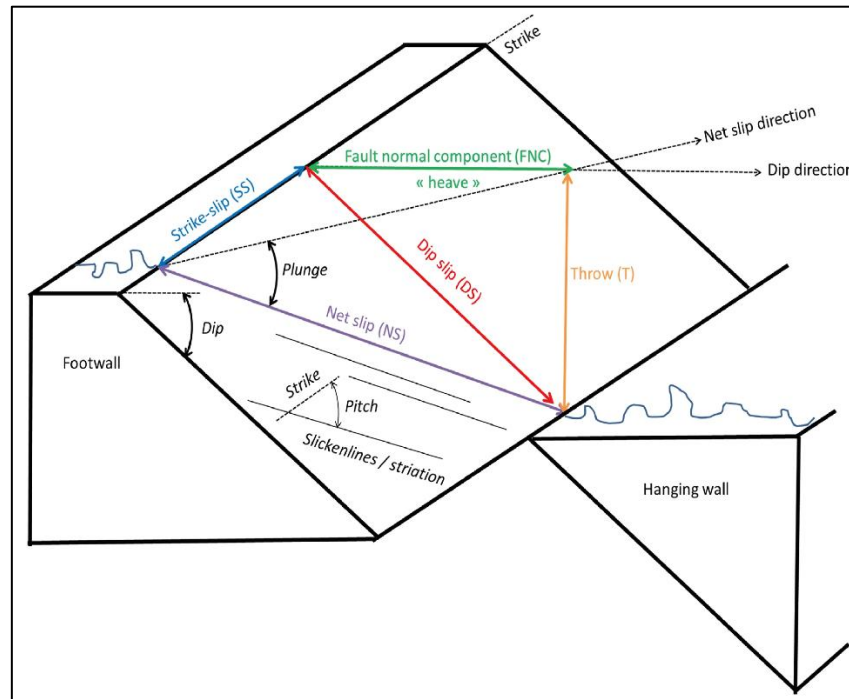
Figure 1-13: Slip components in FDHA (taken from Nurminen et al., 2022; Figure 2).
