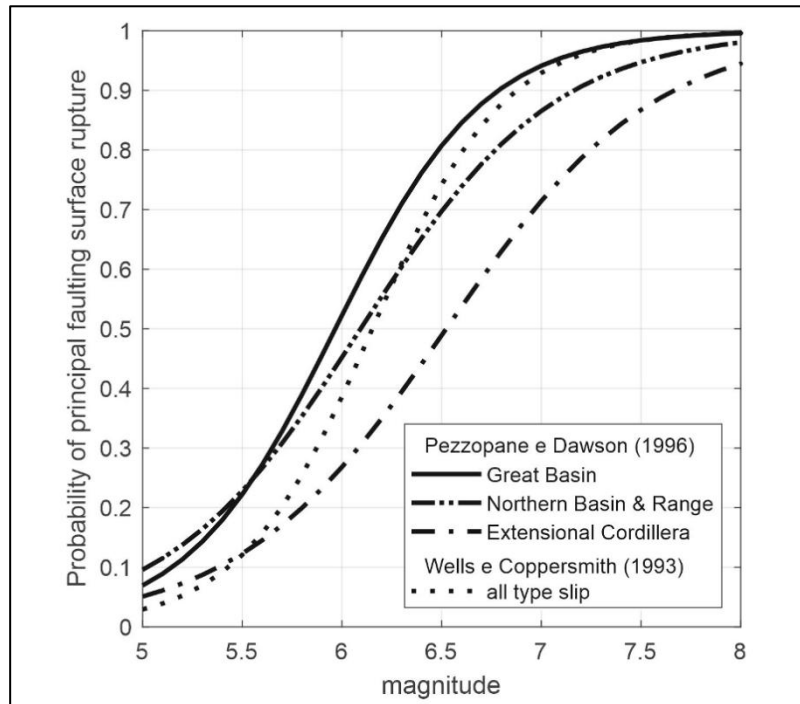
Figure 1-3: Conditional probability of occurrence of principal surface rupture obtained from the logistic regression and the various databases indicated (taken from Youngs et al., 2003; Figure 4).
