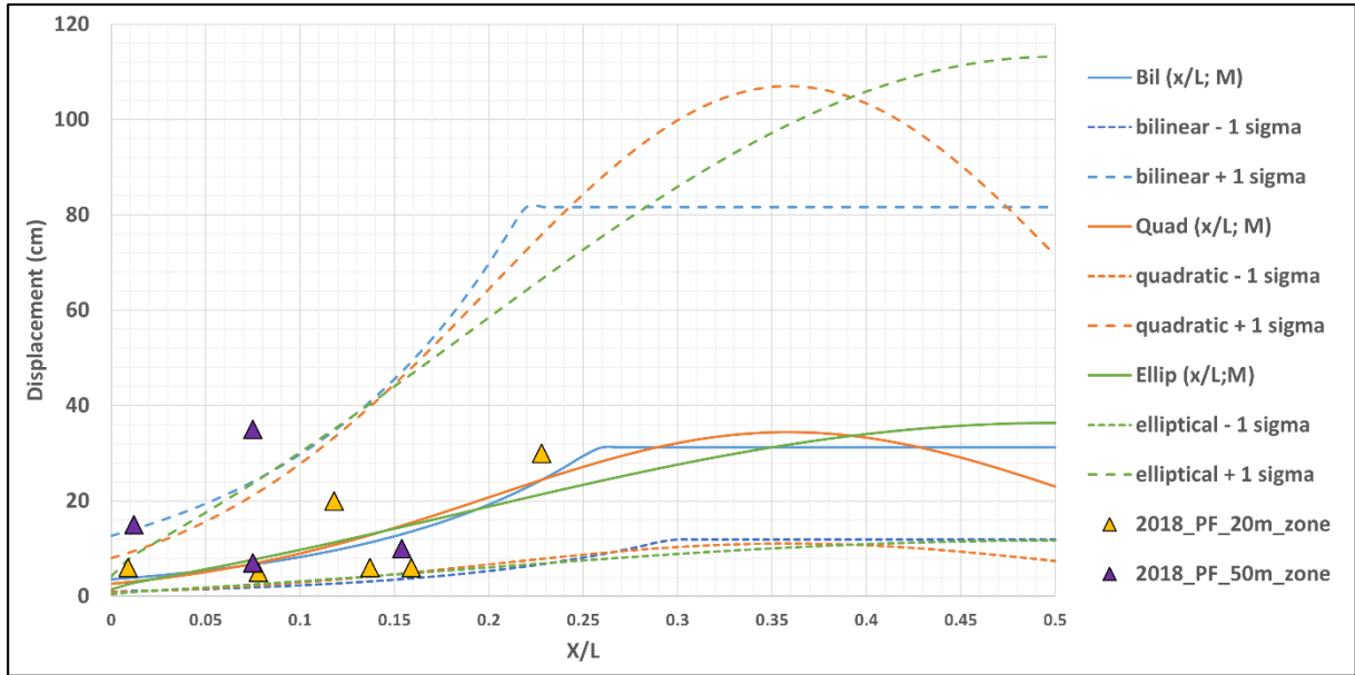
Figure 2-10: Comparison of the principal horizontal displacement observed along the Milun fault during the 2018 Hualien earthquake with the PEA11 models.
