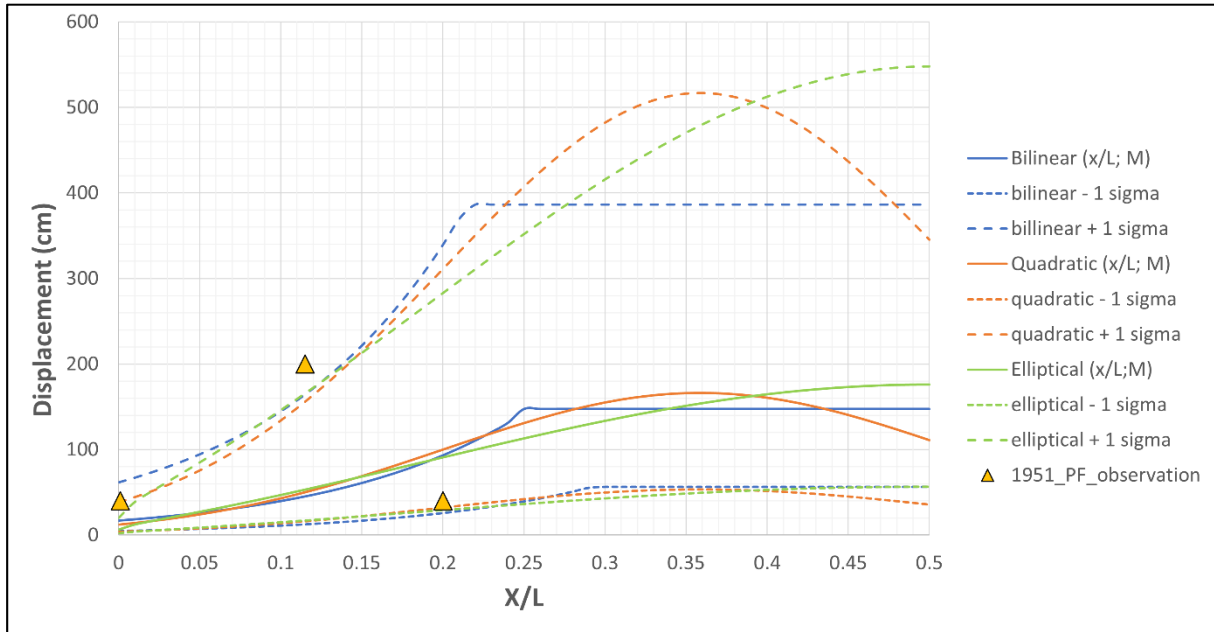
Figure 2-6: Comparison of the principal horizontal displacement observed along the Milun fault during the 1951 Hualien earthquake with the PEA11 models.
