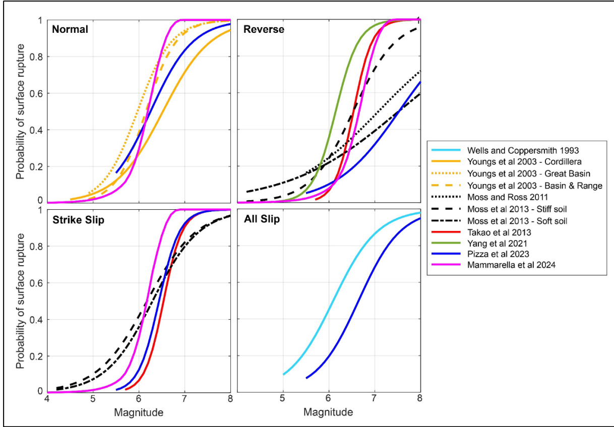
Figure 1-9: Probability of principal surface rupture for various faulting styles and multiple datasets (taken from Valentini et al., 2025; Figure 10).
