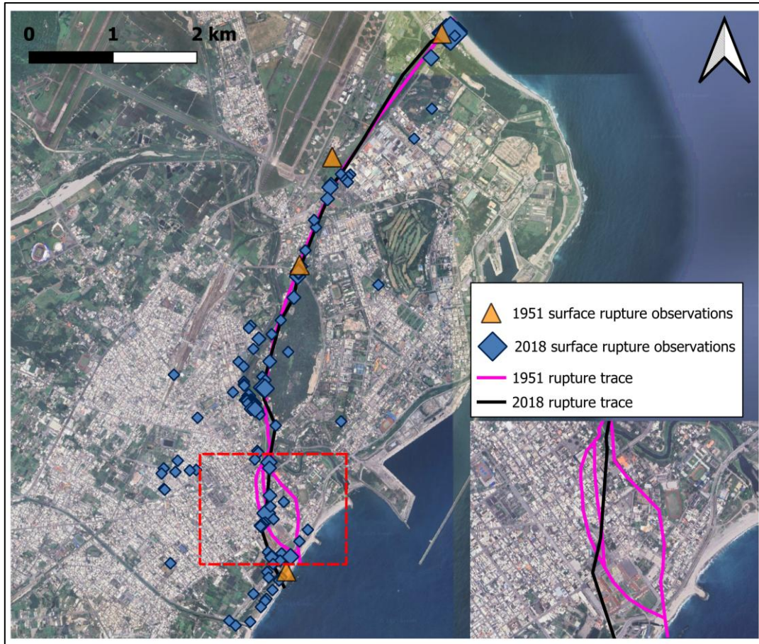
Figure 2-4: Rupture traces and surface displacement data of the 1951 and 2018 Hualien earthquakes.
