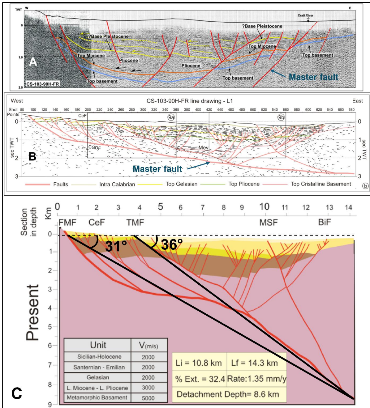
Figure 3-15: Interpretation of a seismic line across the central part of the Crati Valley. (modified from: A) Spina et al., 2011; B) Brozzetti et al., 2017b. C) Seismic section transformed in depth (modified from Brozzetti et al., 2017b)
