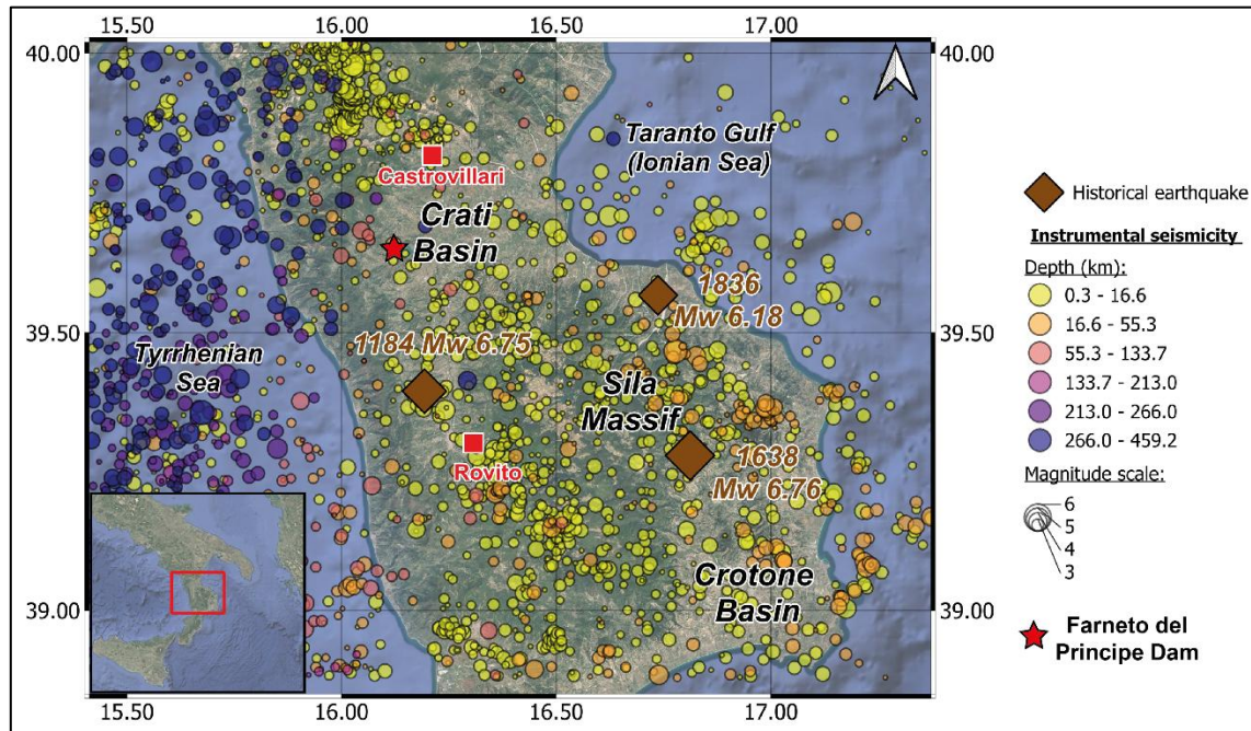
Figure 3-1: Seismicity map of the study area, in Calabria region, Italy (inset map). The instrumental earthquakes (coloured circles) are taken from the ISIDe Working Group (2007), ( M \geq 2.5 ; 1980–2025); the main historical events (brown rhombs) taken from CPTI15 (Rovida et al., 2020) are labelled by date and magnitude. By red squares two specific locations we investigated.
