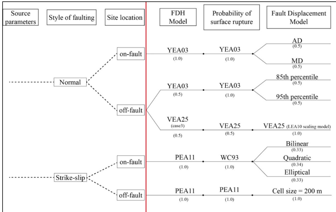
Figure 3-29: Logic flow used for fault displacement hazard map calculations. On the left of the red line, alternative choices are site-dependent; on the right, different branches of the logic-tree approach are modelled for all the sites. WC93 stays for Wells and Coppersmith, 1993; LEA10 for Leonard et al., 2010 (both applied for
