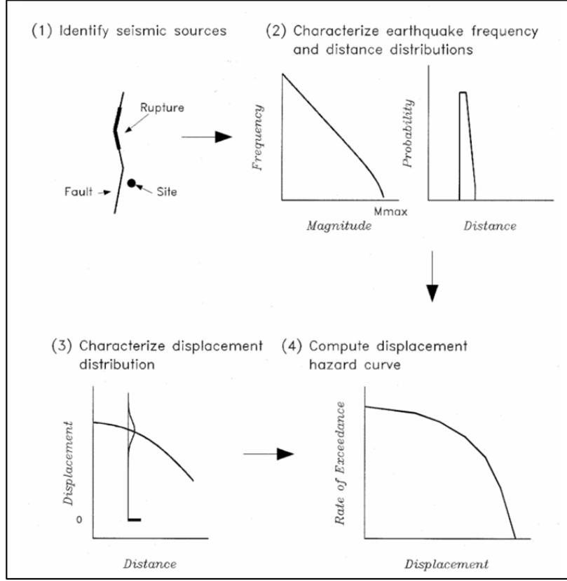
Figure 1-2: Simplified scheme illustrating the PFDHA earthquake approach steps (from Youngs et al., 2003; Figure 2)
