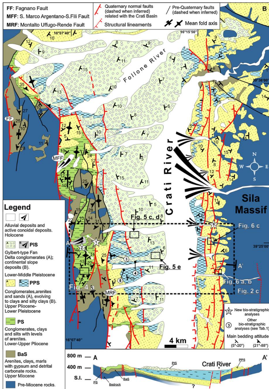
Figure 3-14: Geological map of the Crati Valley (from Spina et al., 2011; Figure 3b)
