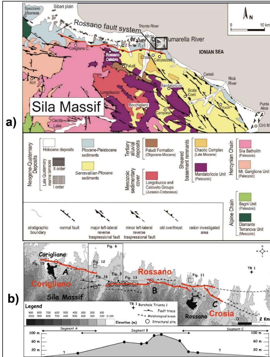
Figure 3-16: Rossano fault system. a) Geo-structural map of the northern part of the Sila Massif (modified from Gori et al., 2016); b) Rossano fault segmentation with Corigliano, Rossano and Crosia segments (modified from Galli et al., 2010)
