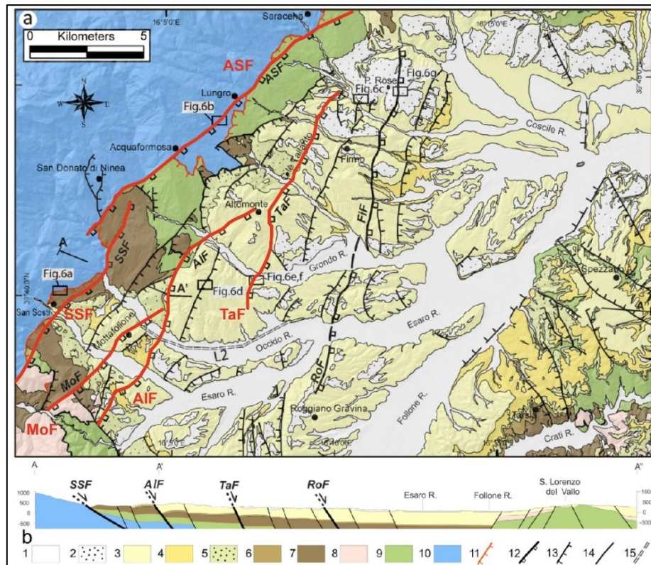
Figure 3-12: Fault segments located in the northern part of the Crati Valley (modified from Brozzetti et al., 2017a)
