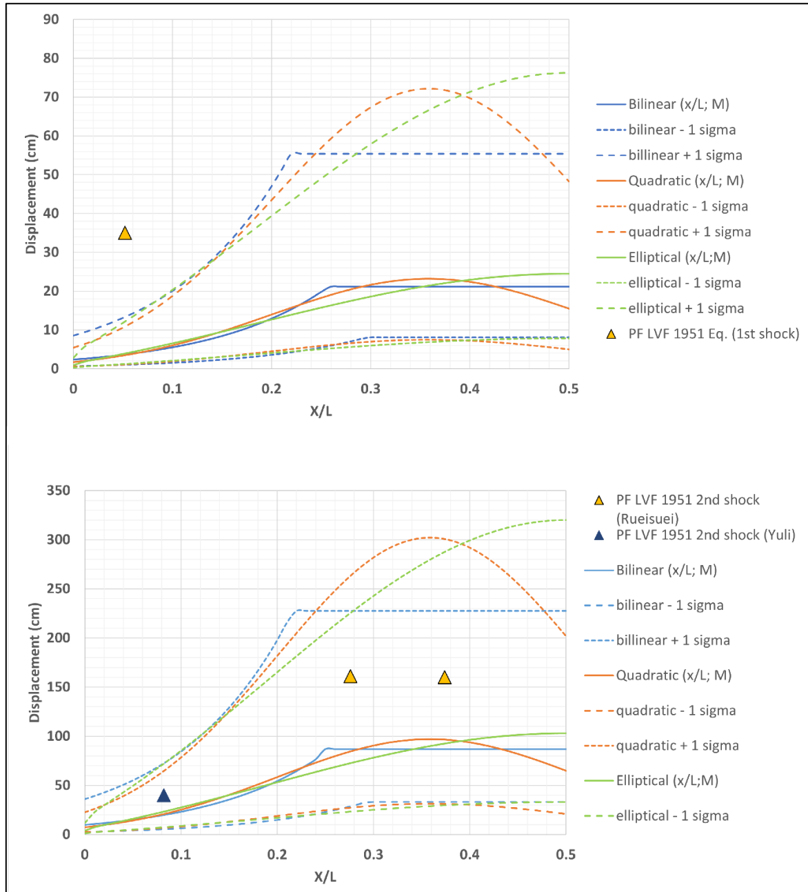
Figure 2-18: Comparison of the principal horizontal displacement observed along the LV during Taitung 1951 1st shock (top) and 2 nd shock (bottom) with the PEAI1 models.
