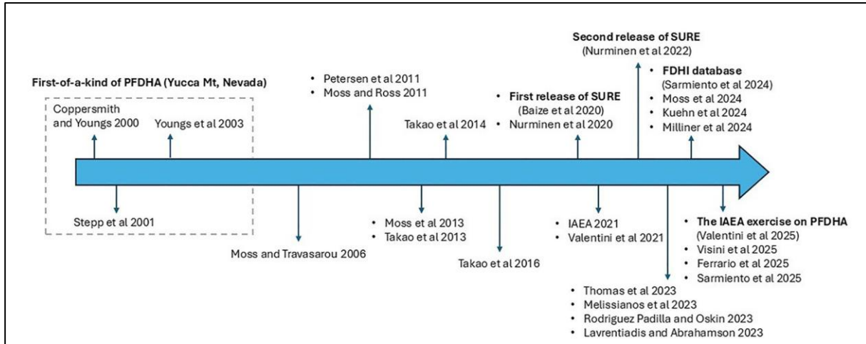
Figure 1-8: Overview of the key PFDHA models published in the literature up to 2025 (taken from Valentini et al. (2025), Figure 1).
