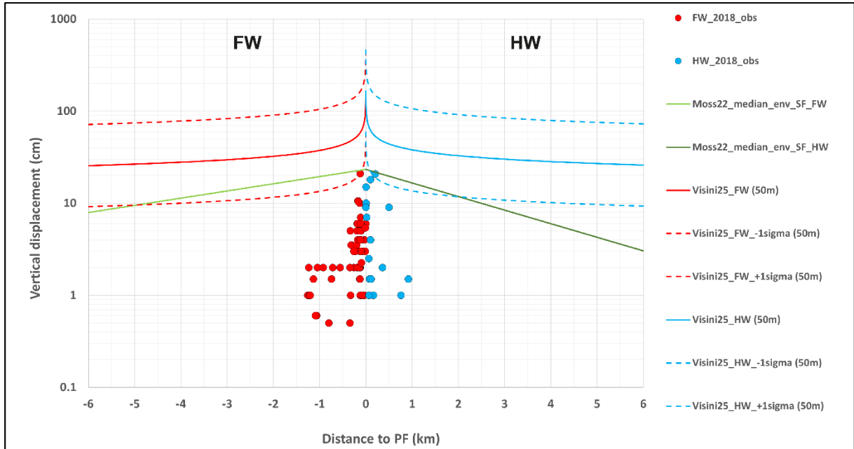
Figure 2-13: Comparison of the distributed vertical surface displacement observed during the 2018 Hualien earthquake with empirical regressions from MEA22 (Moss22) and VEA25 (Visini25) (HW: hanging wall, FW: foot wall).
