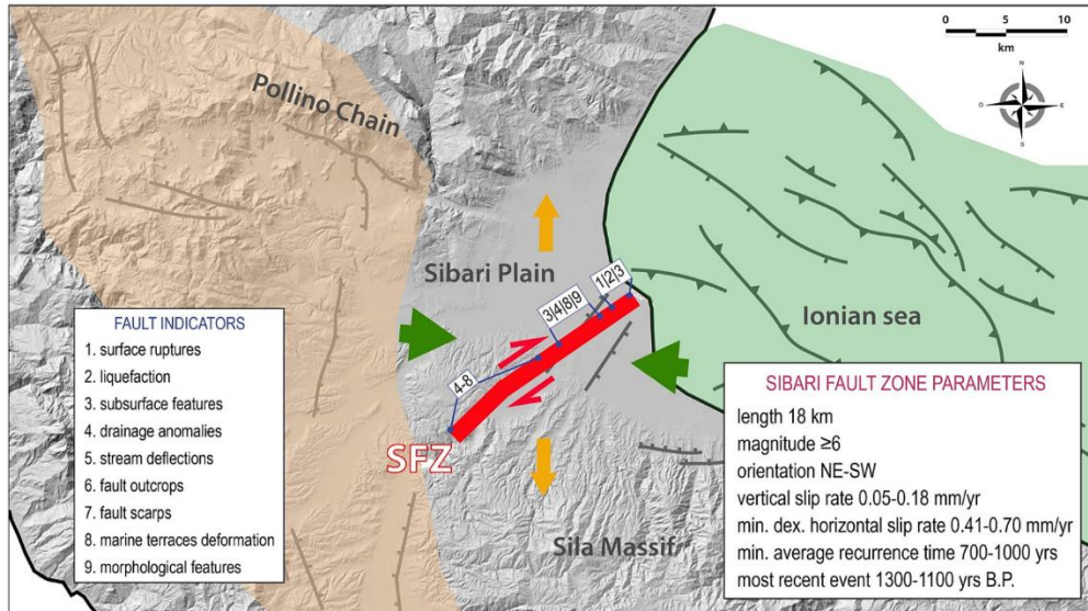
Figure 3-10: Sibari Fault Zone (from Cinti et al., 2024; Figure 18)
