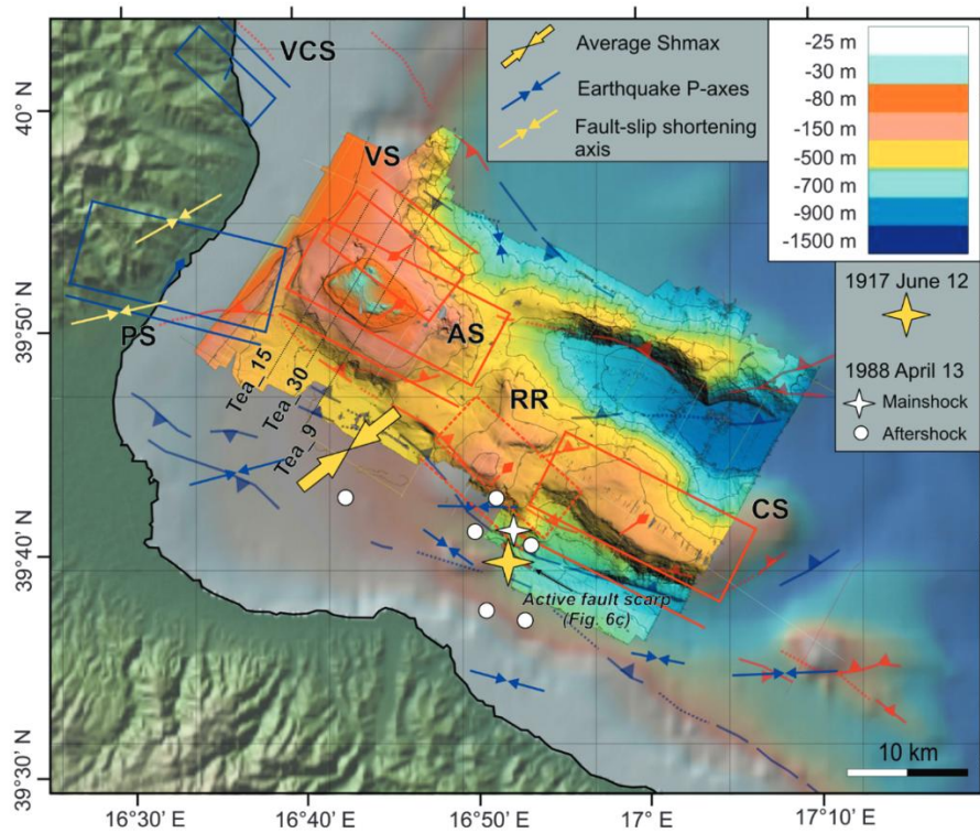
Figure 3-11: Tectonic map of the Amendolara ridge, in the Gulf of Taranto. Amendolara fault system proposed by Ferranti et al., 2014; with AS: Amendolara segment; VS: Valsinni segment; CS: Cariati segment.
