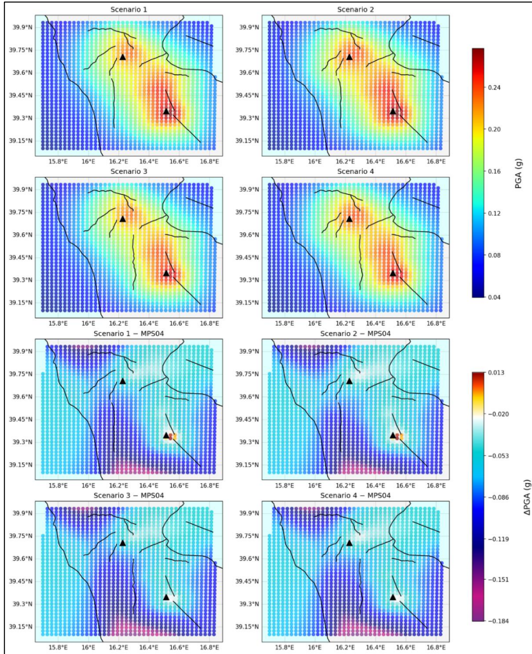
Figure 3-27: Seismic hazard maps derived from our fault model for northern Calabria. The top four panels show the four fault-configuration scenarios (PGA, 10% probability of exceedance in 50 years), while the bottom four illustrate the differences relative to the MPS04 dataset (Meletti et al., 2006).
