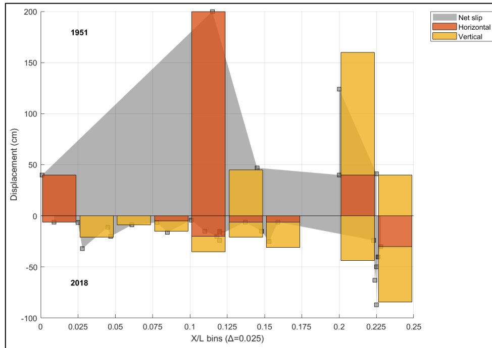
Figure 2-5: Comparison of the average fault displacement observed along the Milun fault during the 1951 and 2018 Hualien earthquakes.
