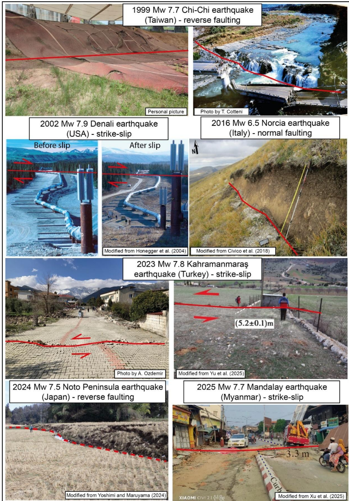
Figure 1-1: Collection of surface rupture photographs around the world, taken in various places and kinematic contexts.
