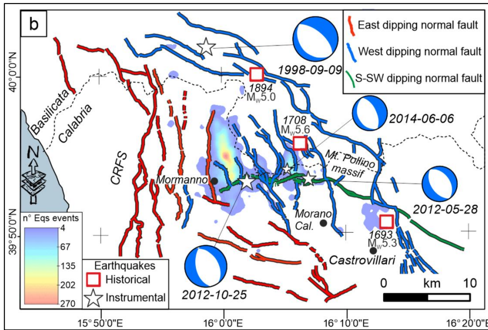
Figure 3-8: Faults in the Pollino chain (from Cirillo et al., 2022; Figure 1b). The PFZ is shown in green.
