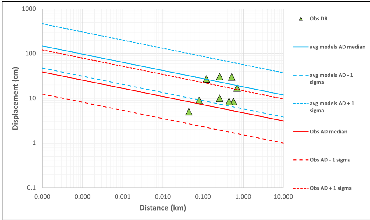
Figure 2-22: Comparison of the distributed horizontal displacement observed during the 2022 Chihshang earthquake with PEAI1 model. In red, AD is obtained from the data; in blue using empirical regressions.
