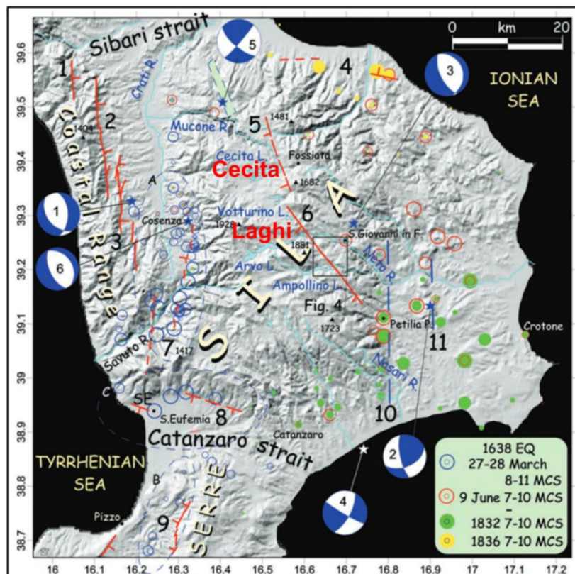
Figure 3-17: Potential active faults in the Sila Massif (modified from Galli and Bosi, 2003)
