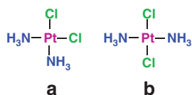
Scheme 1: Cisplatin (a) and transplatin (b).
