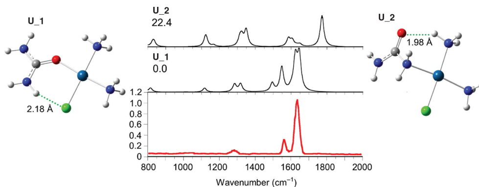
Fig. 3: IRMPD spectrum of cis -[PtCl(NH 3 ) 2 (Urea)] + (red profile) compared with calculated harmonic IR spectra of U_1 and U_2 isomers optimized at the B3LYP/6-311+G(d,p) (Pt=LANL2TZ) level (black profiles). Relative free energy at 298 K, in kJ mol -1 , is given under each U_1/2 label. Theoretical spectra are scaled by a 0.974 factor.
