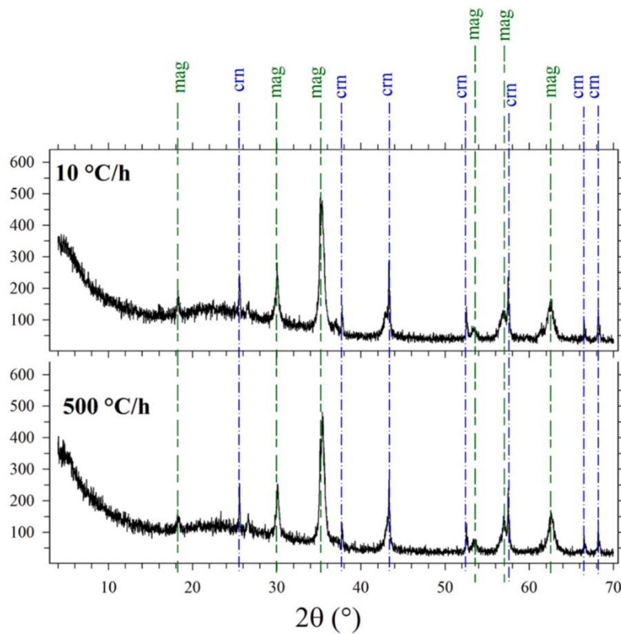
Fig. 2. XRPD spectra of the samples solidified at 10 and 500 °C/h, acquired with a X'Pert PRO from 4 to 70°, with a step scan of 8 s each 0.02° of 2θ. The most intense Bragg reflections correspond to standard crystalline phases of magnetite (mag); corundum (cm) was used as internal standard.
