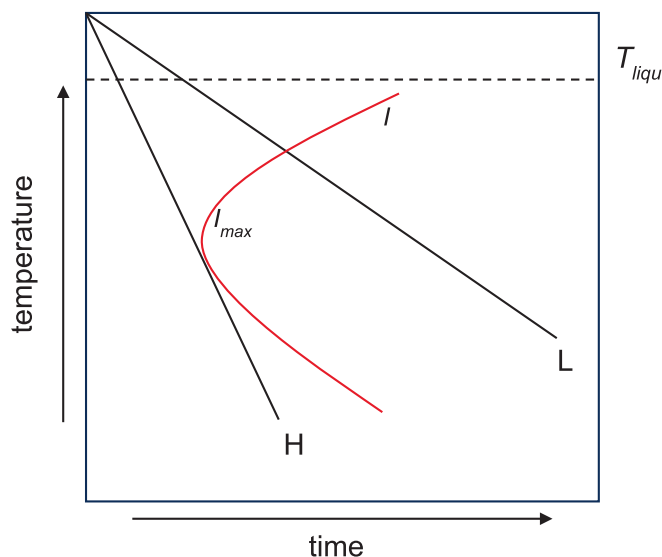
Fig. 5. Schematic temperature–time–transformation (TTT) diagram. The red curve represents the nucleation rate I , the T_{\text{liqu}} the liquidus temperature and the H and L black lines the intermediate (500 °C/h) and the low (10 °C/h) cooling rates; the nose or the tip of the red curve corresponds to I_{\text{max}} , maximum nucleation rate. (For interpretation of the references to colour in this figure legend, the reader is referred to the web version of this article.)
