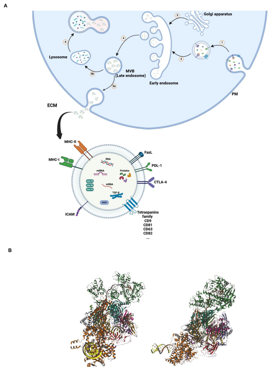
Figure 1. (A) Mechanism of synthesis and release of EVs. Inward budding of plasma membrane (PM) toward cytosol led to the formation of early endosome (1 and 2); communication between early endosome and Golgi apparatus formed and released late endosome or multivesicular bodies (MVB) (3 and 4); upon fusion of MVB with PM, exosomes are released into the ECM (5a); combination of MVB with lysosome result in degradation of MVB in cytosol (5b and 6). (B) Three-dimensional structural views of the human nuclear exosome-MTR4 RNA complex. (The structure is publicly available at the link: https://www.rcsb.org/3d-view/6D6Q/1 , accessed on 6 March 2024).
