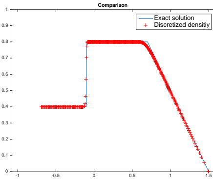
FIGURE 2. Comparison between the exact solution (continuous blue line in the pdf version of the paper) and \rho^n(t, x) (“+” in red in the pdf version of the paper) for N = 400 particles and initial datum (10).
