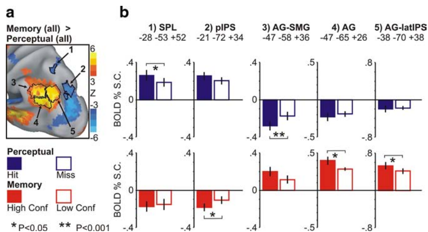
Figure 5. Relation between behavioral performance and search-related activity in the left parietal lobe. a , Multiple-comparison corrected z -map of the contrast between memory and perceptual search-related activity, in which the search parameters corresponding to different behavioral outcomes were collapsed, avoiding ROI selection biases. b , Graphs showing the BOLD percentage signal change for search parameters corresponding to different behavioral outcomes: high (full bar) and low (empty bar) confidence correct trials in the memory task (red bars), hits and misses in the perceptual task (blue bars). These parameter magnitudes were obtained from a . Regions of the left parietal lobe (illustrated in a , 1–5) more activated by perceptual (1, 2) and by memory (3–5) search are presented. Error bars indicate SEM. Asterisks represent the significance of the two-tailed paired t test between search parameters in the same task.
