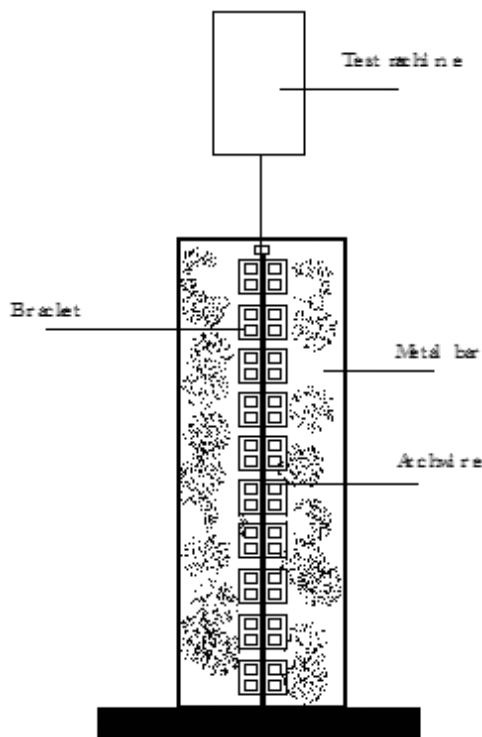
FIGURE 1. Testing model and mechanical testing machine.
