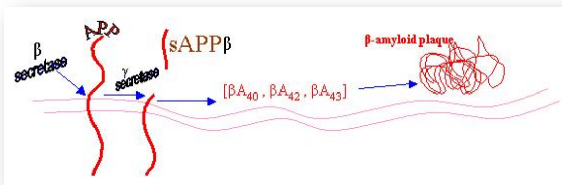
Fig. (1). Illustration of abnormal protein processing in AD. (APP, amyloid precursor protein; \beta A, \beta -amyloid).
