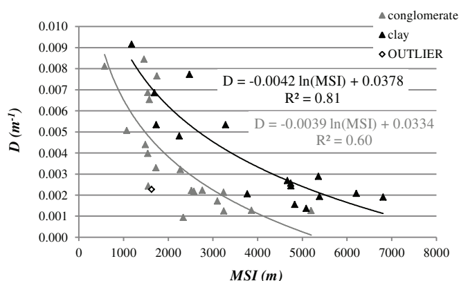
Figure 2. Regression between D and MSI of TINITALY data with distinction of basins' lithology (manly conglomerate in grey, mainly clay in black).
