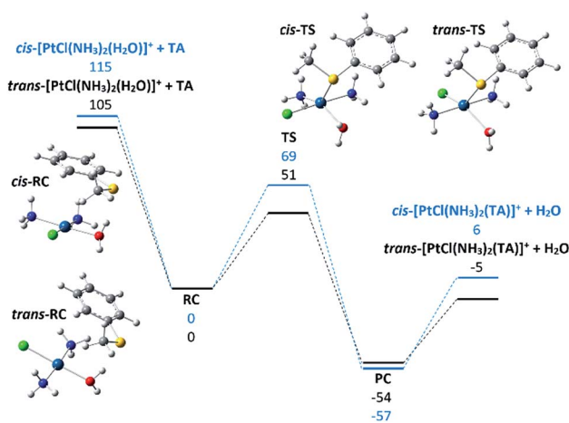
Fig. 4 Computed profile for the reaction of cis - and trans - [\text{PtCl}(\text{NH}_3)_2(\text{H}_2\text{O})]^+ with TA. Optimized geometries of the reactant collision complexes ( cis - and trans - [\text{PtCl}(\text{NH}_3)_2(\text{H}_2\text{O})]^+ \cdot \text{TA} ) and of the transition states TS are shown. Relative enthalpies at 298 K (kJ mol -1 ) are reported.
