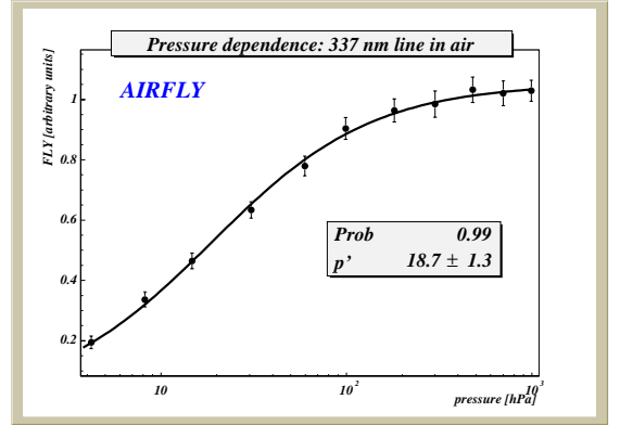
Figure 2. Pressure dependence of the 337 nm line in Air
