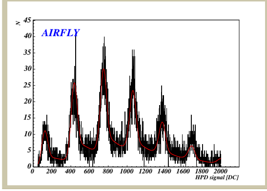
Figure 1. HPD single photoelectron spectrum.
