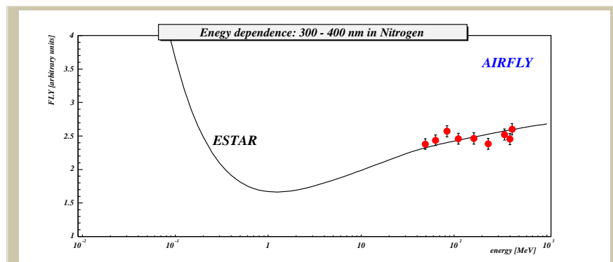
Figure 4. Energy dependence of FLY in Nitrogen
