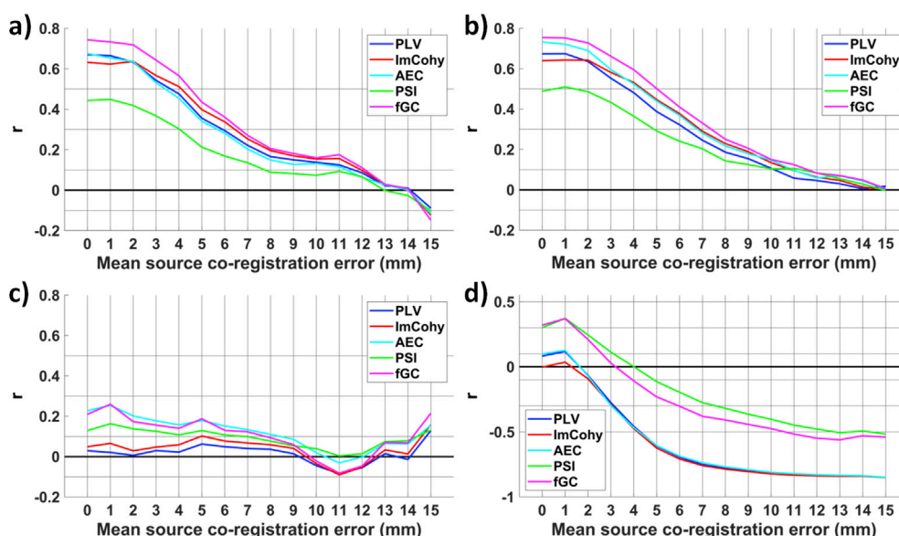
Fig. 7. a–c) Effect size r for the difference between RE distributions obtained by using different TMs (i.e., a) RE_{TM-3c} - RE_{TM-4c} ; b) RE_{TM-1c} - RE_{TM-4c} ; c) RE_{TM-1c} - RE_{TM-3c} ) with beamforming source reconstruction, as a function of the mean source co-registration error. d) Effect size r for the difference between RE distributions obtained by using different source reconstruction techniques, i.e., RE_{MNE} - RE_{beamforming} , with TM-4c, as a function of the mean source co-registration error. Conventional values for a small (0.1), medium (0.3), large (0.5) effect size have been marked by the horizontal grid lines. Different colored lines refer to different connectivity measures (PLV, ImCohy, AEC, PSI, fGC).
