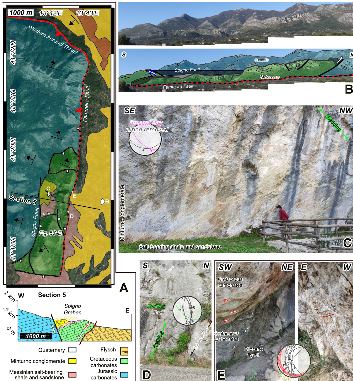
Figure 8. Geology of the Fammera Fault area. (a) Geological map and cross section. (b) Interpreted panoramic photo of the Spigno Graben as seen from the east, representing a natural cross section of the structure. (c) Strike-slip fault mirror in the Minturno conglomerate, with bedding trace indicated in green. Back tilting of strata makes the fault become normal dip-slip. (d) Dip-slip fault in the western damage zone of the Fammera Fault affecting steeply dipping Cretaceous carbonates. (e) Close up views of the Fammera Fault principal displacement zone with plot of structural data, showing low-angle NE-verging thrust cut by high-angle normal faults. Stereographic projections on Schmidt net, lower hemisphere.
