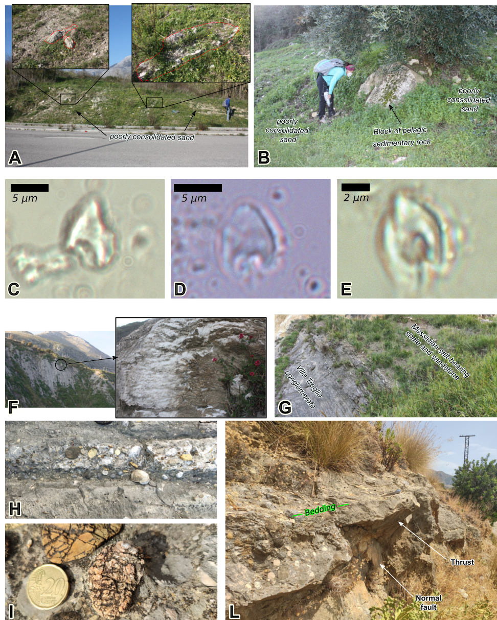
Figure 5. (a) Sedimentary mélanges formed by poorly consolidated sand of the lower portion of the Messinian salt-bearing shales and sandstones, with insets showing m-sized blocks of pelagic limestones (Location 41.274694°N, 13.710114°E). (b) Block of pelagic limestone embedded within poorly consolidated sand of the lower portion of the Messinian salt-bearing shales and sandstones, Spigno section. Microphotographs showing calcareous nannofossils found in the Messinian salt-bearing shales and sandstones: (c) Amaurolithus primus , (d, e) cf. Amaurolithus primus (primitive morphotypes) (samples location in Figure 8a). (f) Panoramic photo and close up view of a Gypsum block at the topmost portion of slightly mixed and disrupted Messinian salt-bearing sandstones and shales in the Villa Treglia section (Location of the block 41.269094°N, 13.613944°E). (g) Conformable stratigraphic contact between the Messinian salt-bearing sandstones and shales and the underlying Villa Treglia Conglomerate in the Villa Treglia section (Location of the contact 41.267289°N, 13.612959°E). (h) Detail of the Villa Treglia Conglomerate showing a conglomerate level sandwiched between two calcarenite levels. (i) Detail of a pink granite clast within the Villa Treglia conglomerate. (l) Gently dipping strata of the Villa Treglia conglomerate affected by a brittle normal fault cutting and displacing a previous brittle thrust (Location of the contact 41.261963°N, 13.611167°E).
