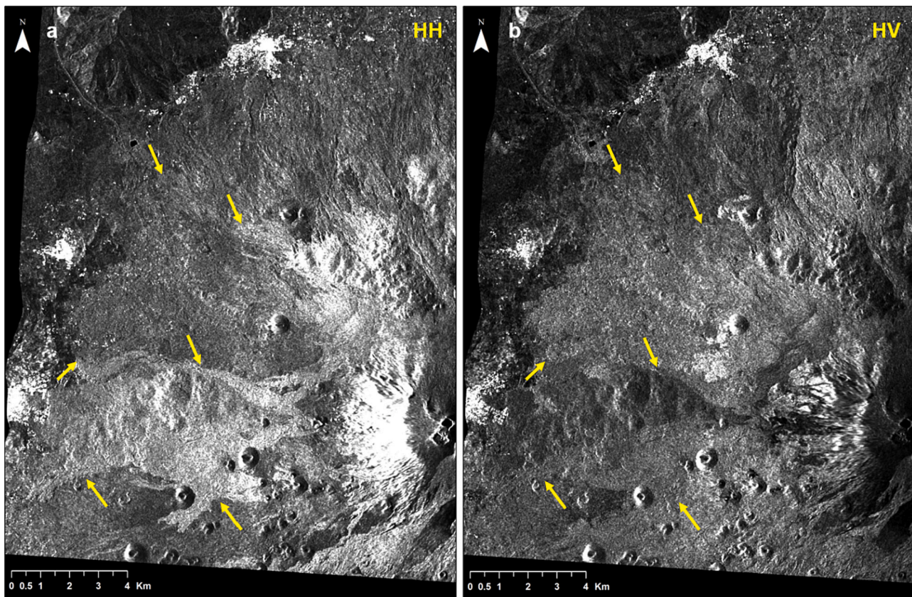
Fig. 5. RISAT-1 A C-band (wavelength 5.3 cm) SAR data of Mt. Etna region shown here in a) HH, b) HV polarizations at 4 m /pixel resolution. Arrows highlight the extents and boundaries of historical and recent lava flows that have a suite of textures (a’ a to pāhoehoe). Notice the high degree of unit discrimination in the HV-pol data compared to the HH-pol data, since the HV-pol echoes are more sensitive to surface roughness at all incidence angles.
