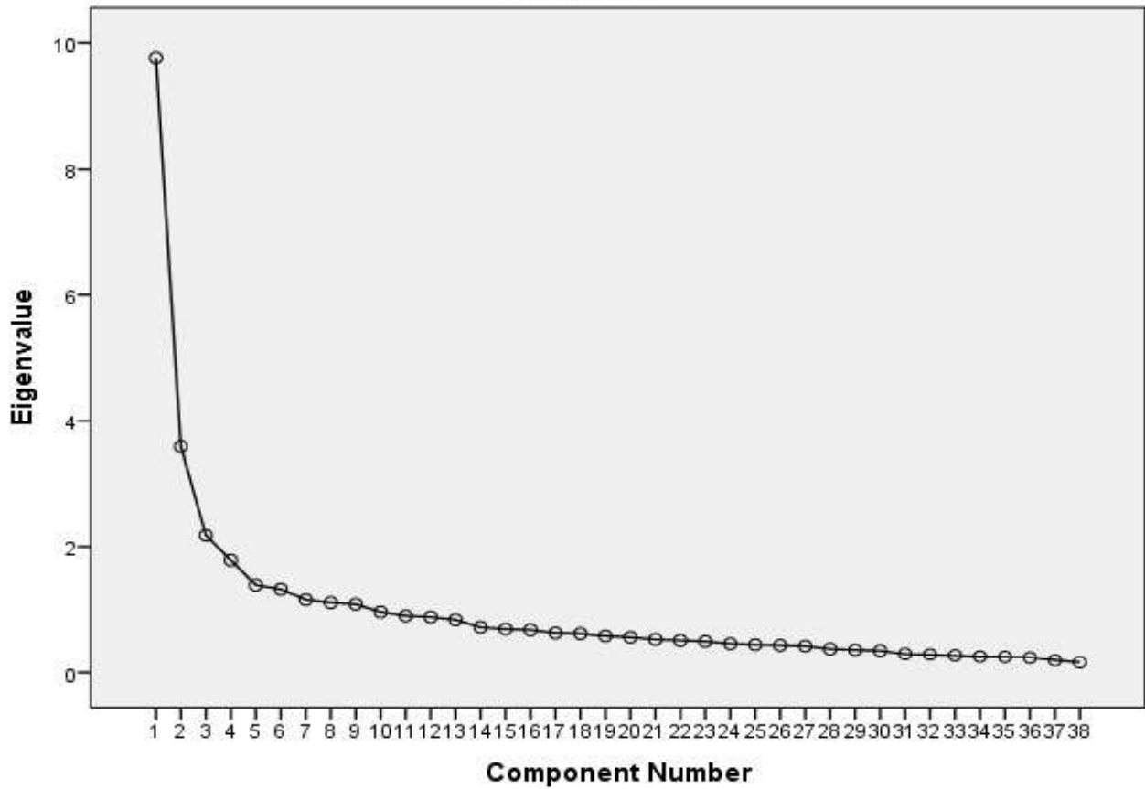
Scree Plot
